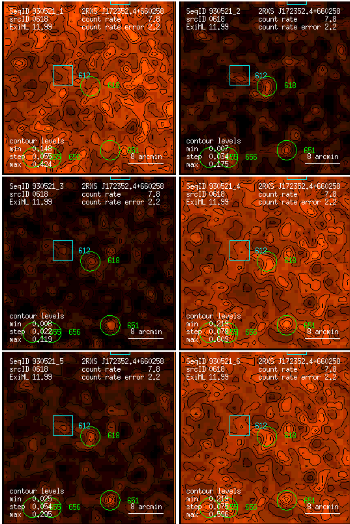
Figure 618: RASS 930521: detection 0618: band rate images, Gaussian filter: (1) PSPC channels 11 – 41, (2) 52 – 90, (3) 91 – 201, (4) 11 – 235, (5) 52 – 201, (6) 11 – 201. Broad band rates in counts/ks. Band rate contour levels in counts/ks/arcmin 2 .
