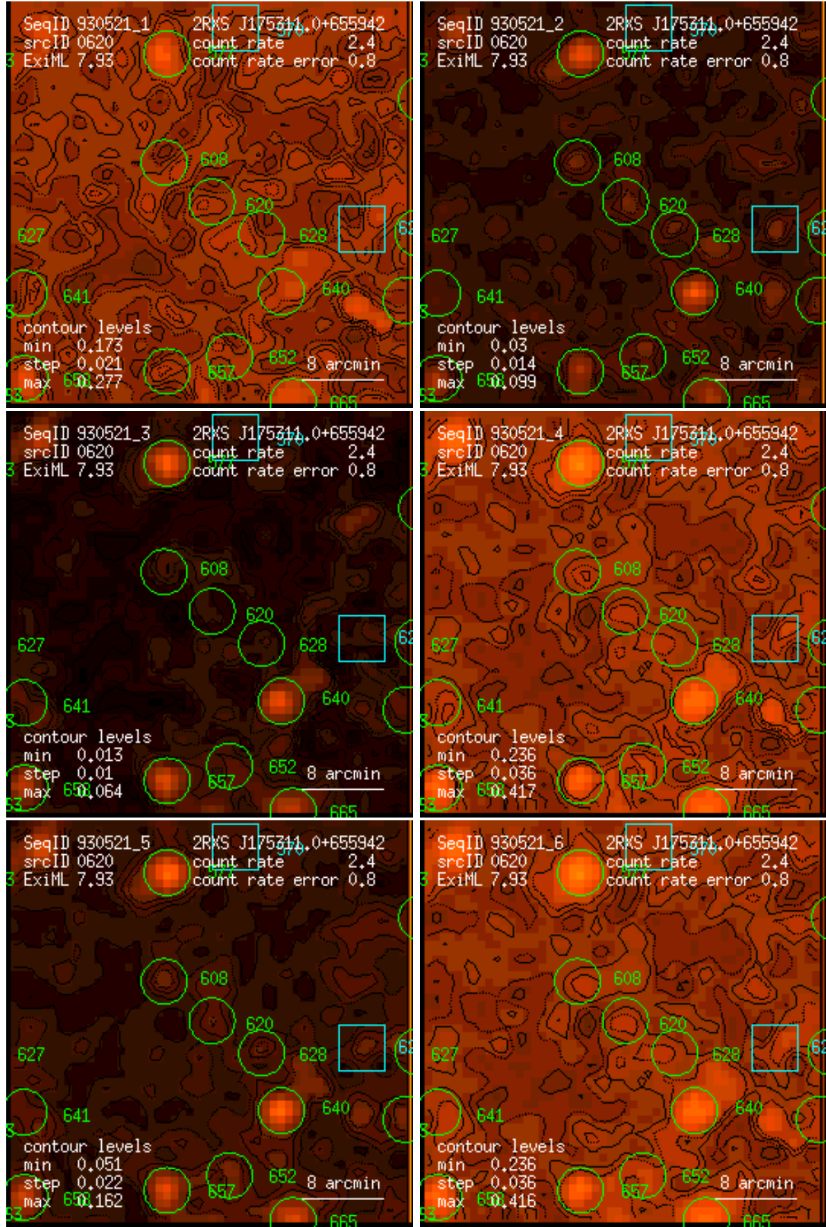
Figure 620: RASS 930521: detection 0620: band rate images, Gaussian filter: (1) PSPC channels 11 – 41, (2) 52 – 90, (3) 91 – 201, (4) 11 – 235, (5) 52 – 201, (6) 11 – 201. Broad band rates in counts/ks. Band rate contour levels in counts/ks/arcmin 2 .
