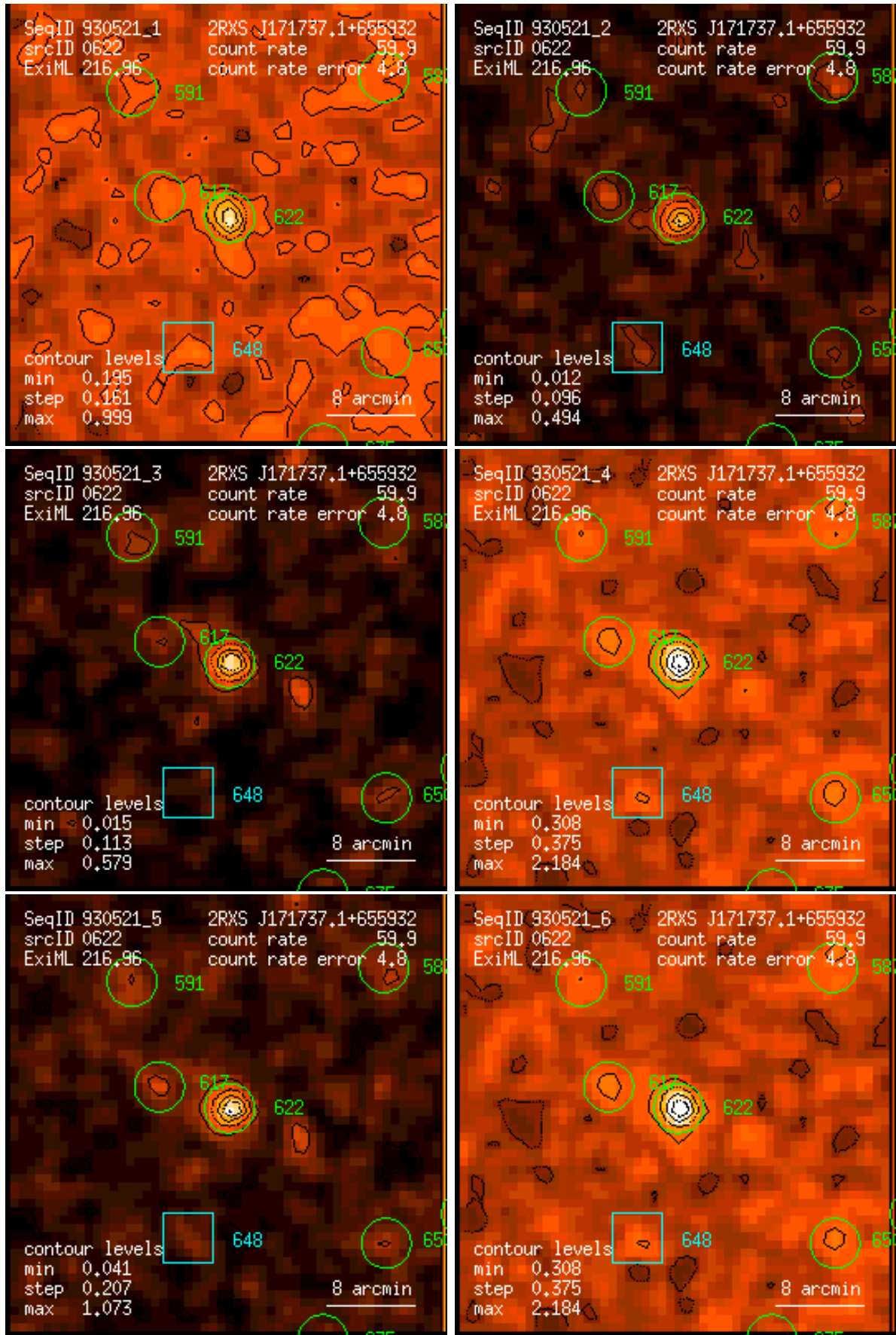
Figure 622: RASS 930521: detection 0622: band rate images, Gaussian filter: (1) PSPC channels 11 – 41, (2) 52 – 90, (3) 91 – 201, (4) 11 – 235, (5) 52 – 201, (6) 11 – 201. Broad band rates in counts/ks. Band rate contour levels in counts/ks/arcmin 2 .
