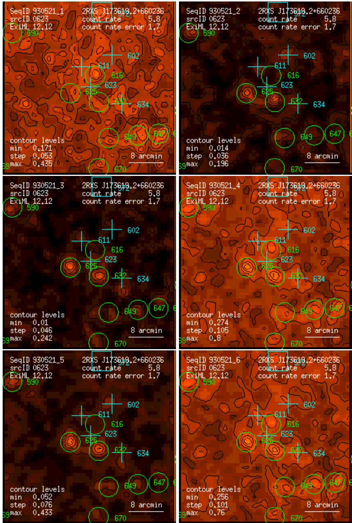
Figure 623: RASS 930521: detection 0623: band rate images, Gaussian filter: (1) PSPC channels 11 – 41, (2) 52 – 90, (3) 91 – 201, (4) 11 – 235, (5) 52 – 201, (6) 11 – 201. Broad band rates in counts/ks. Band rate contour levels in counts/ks/arcmin 2 .
