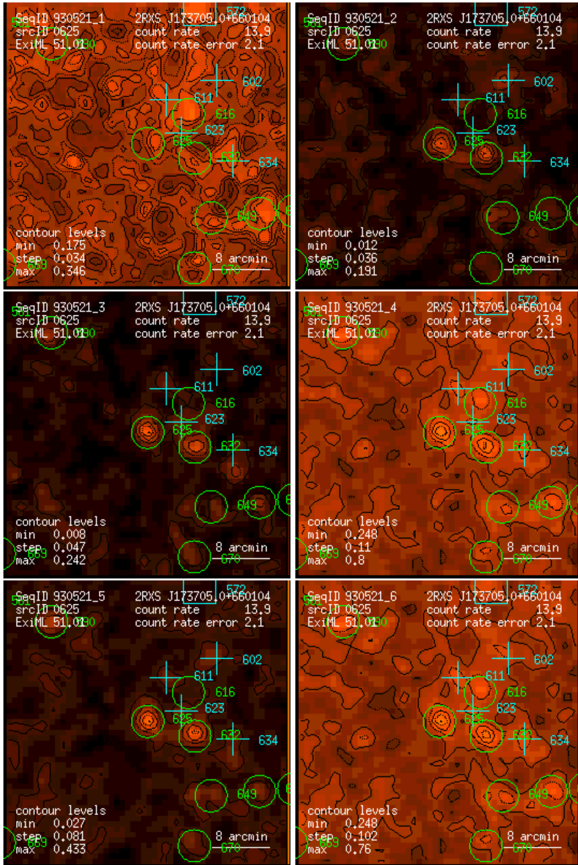
Figure 625: RASS 930521: detection 0625: band rate images, Gaussian filter: (1) PSPC channels 11 – 41, (2) 52 – 90, (3) 91 – 201, (4) 11 – 235, (5) 52 – 201, (6) 11 – 201. Broad band rates in counts/ks. Band rate contour levels in counts/ks/arcmin 2 .
