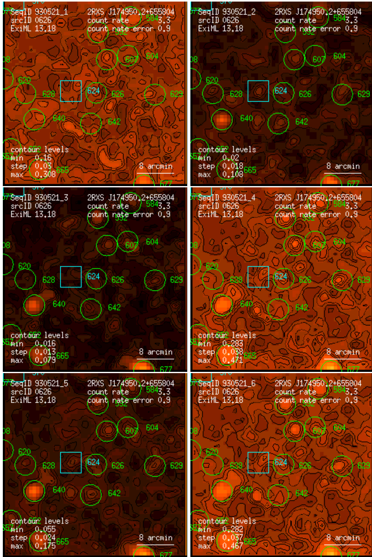
Figure 626: RASS 930521: detection 0626: band rate images, Gaussian filter: (1) PSPC channels 11 – 41, (2) 52 – 90, (3) 91 – 201, (4) 11 – 235, (5) 52 – 201, (6) 11 – 201. Broad band rates in counts/ks. Band rate contour levels in counts/ks/arcmin 2 .
