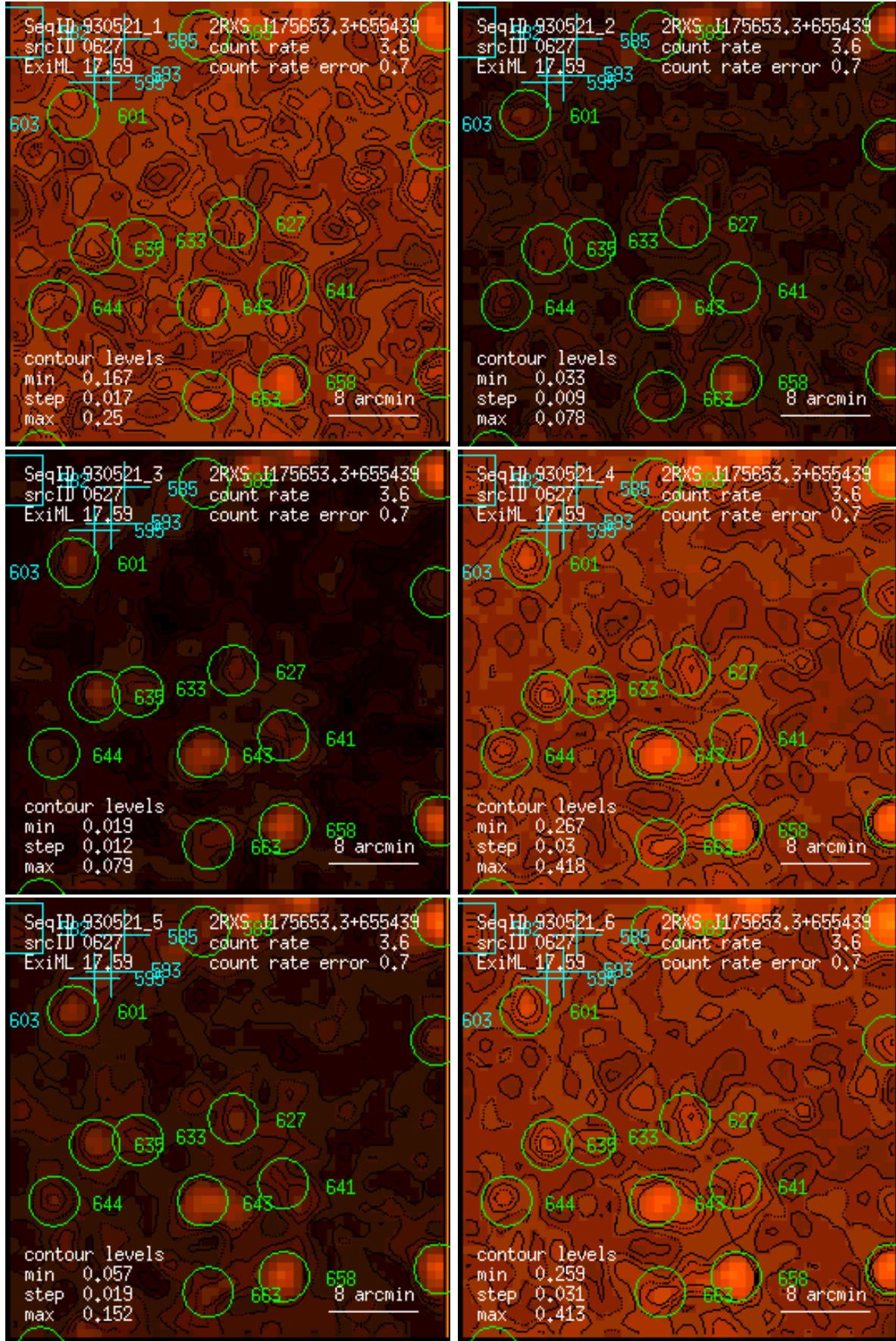
Figure 627: RASS 930521: detection 0627: band rate images, Gaussian filter: (1) PSPC channels 11 – 41, (2) 52 – 90, (3) 91 – 201, (4) 11 – 235, (5) 52 – 201, (6) 11 – 201. Broad band rates in counts/ks. Band rate contour levels in counts/ks/arcmin 2 .
