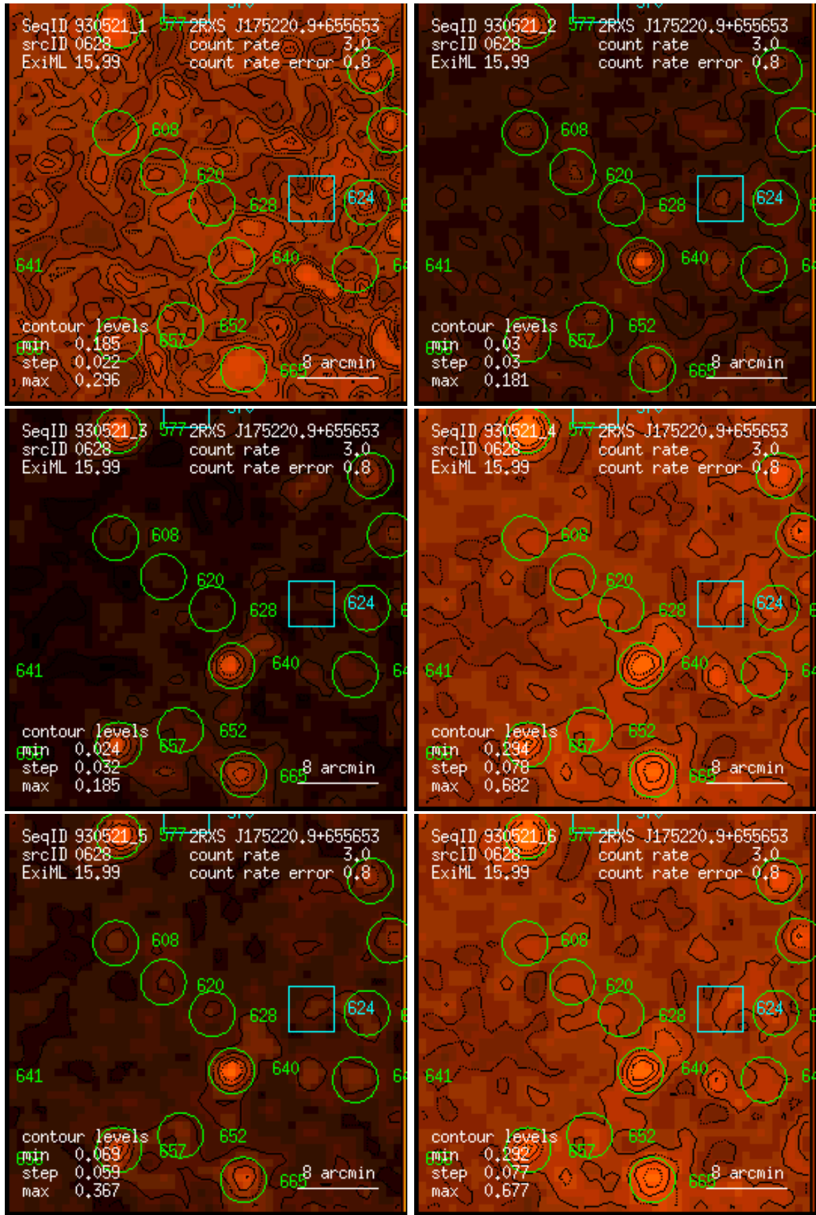
Figure 628: RASS 930521: detection 0628: band rate images, Gaussian filter: (1) PSPC channels 11 – 41, (2) 52 – 90, (3) 91 – 201, (4) 11 – 235, (5) 52 – 201, (6) 11 – 201. Broad band rates in counts/ks. Band rate contour levels in counts/ks/arcmin 2 .
