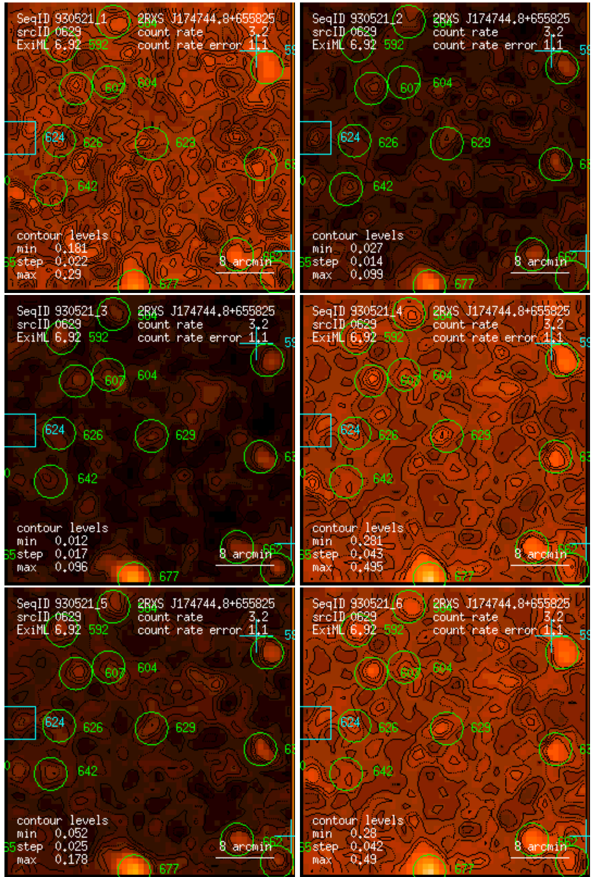
Figure 629: RASS 930521: detection 0629: band rate images, Gaussian filter: (1) PSPC channels 11 – 41, (2) 52 – 90, (3) 91 – 201, (4) 11 – 235, (5) 52 – 201, (6) 11 – 201. Broad band rates in counts/ks. Band rate contour levels in counts/ks/arcmin 2 .
