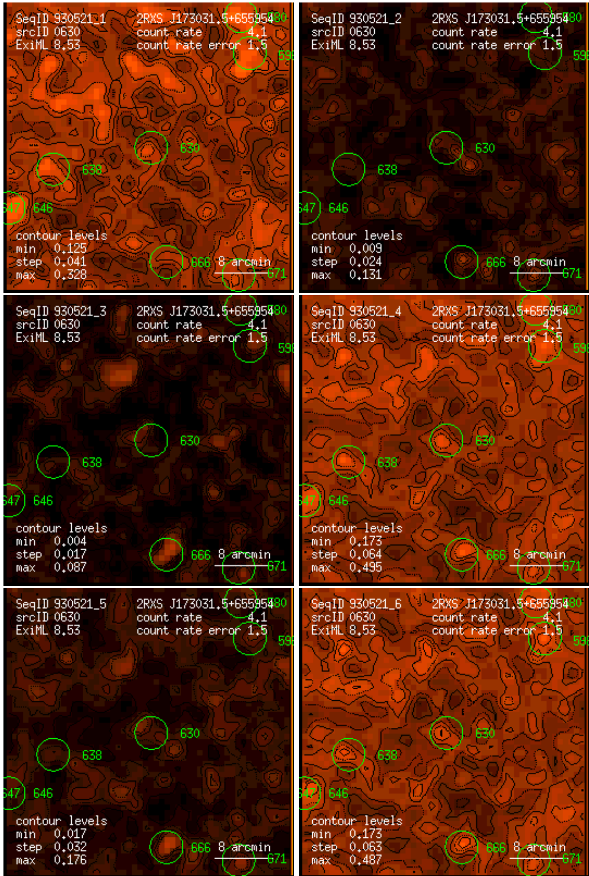
Figure 630: RASS 930521: detection 0630: band rate images, Gaussian filter: (1) PSPC channels 11 – 41, (2) 52 – 90, (3) 91 – 201, (4) 11 – 235, (5) 52 – 201, (6) 11 – 201. Broad band rates in counts/ks. Band rate contour levels in counts/ks/arcmin 2 .
