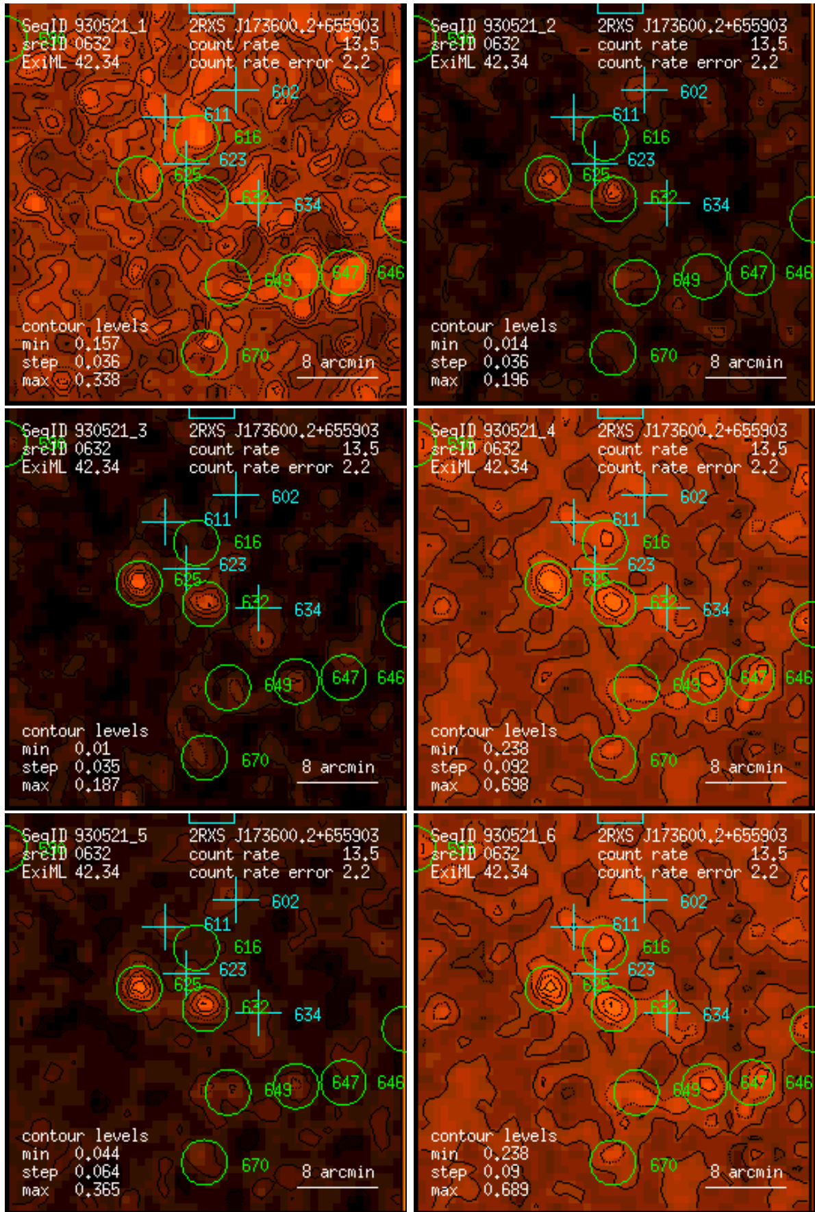
Figure 632: RASS 930521: detection 0632: band rate images, Gaussian filter: (1) PSPC channels 11 – 41, (2) 52 – 90, (3) 91 – 201, (4) 11 – 235, (5) 52 – 201, (6) 11 – 201. Broad band rates in counts/ks. Band rate contour levels in counts/ks/arcmin 2 .
