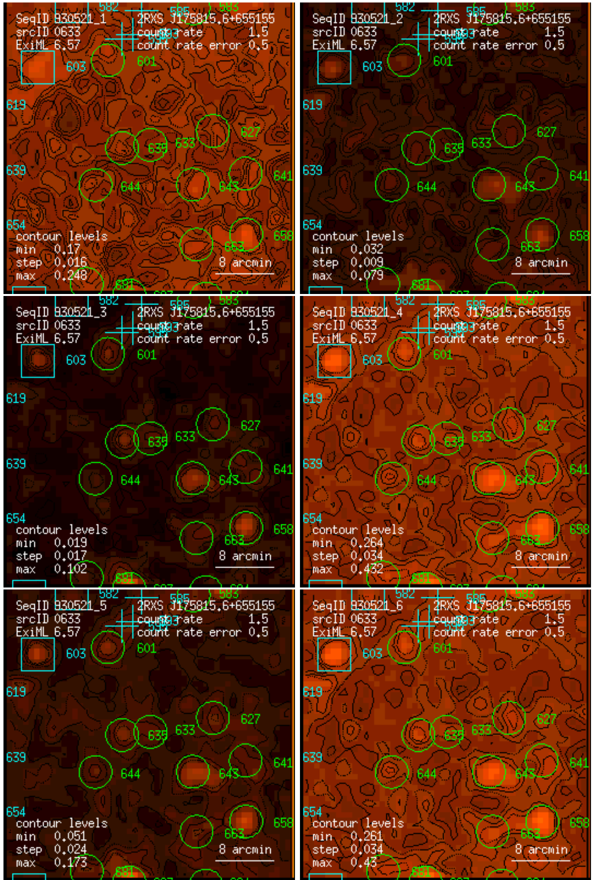
Figure 633: RASS 930521: detection 0633: band rate images, Gaussian filter: (1) PSPC channels 11 – 41, (2) 52 – 90, (3) 91 – 201, (4) 11 – 235, (5) 52 – 201, (6) 11 – 201. Broad band rates in counts/ks. Band rate contour levels in counts/ks/arcmin 2 .
