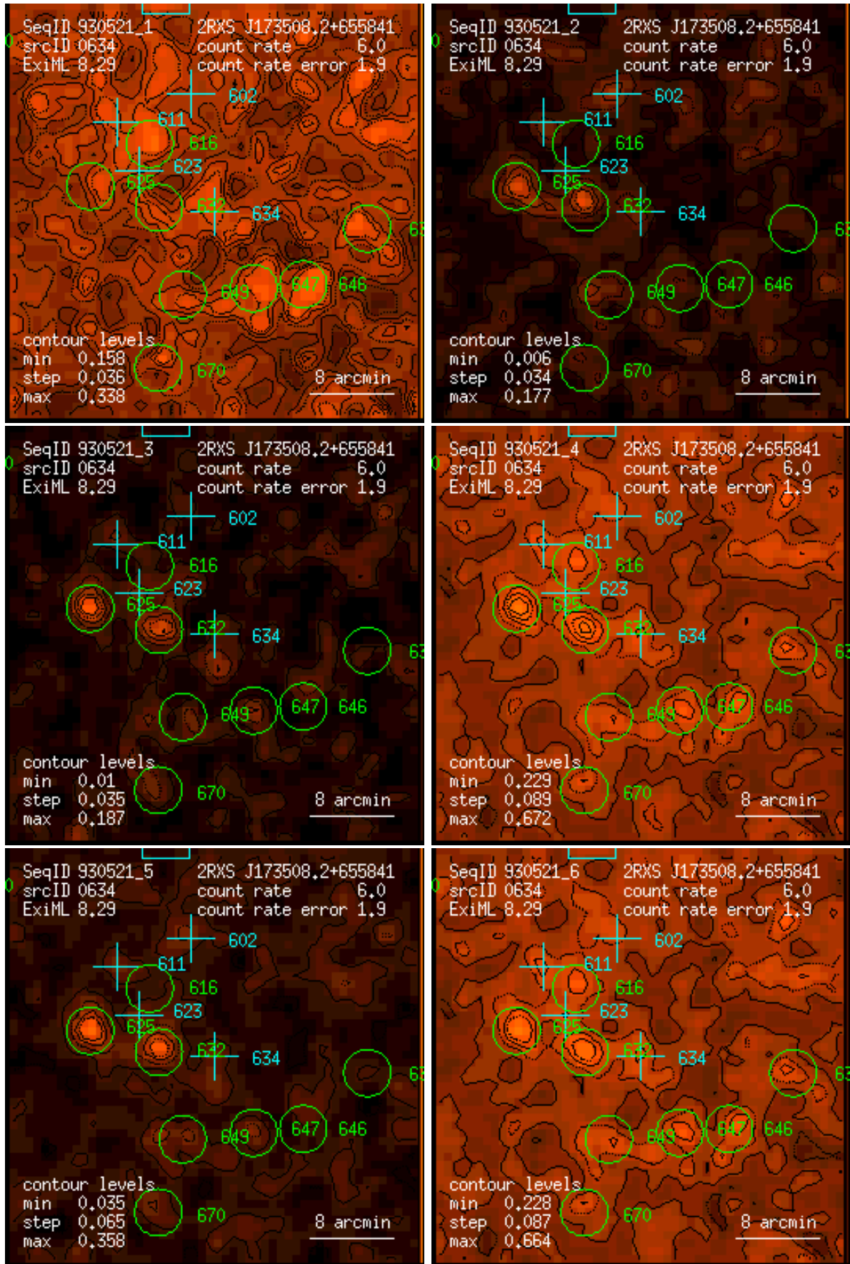
Figure 634: RASS 930521: detection 0634: band rate images, Gaussian filter: (1) PSPC channels 11 – 41, (2) 52 – 90, (3) 91 – 201, (4) 11 – 235, (5) 52 – 201, (6) 11 – 201. Broad band rates in counts/ks. Band rate contour levels in counts/ks/arcmin 2 .
