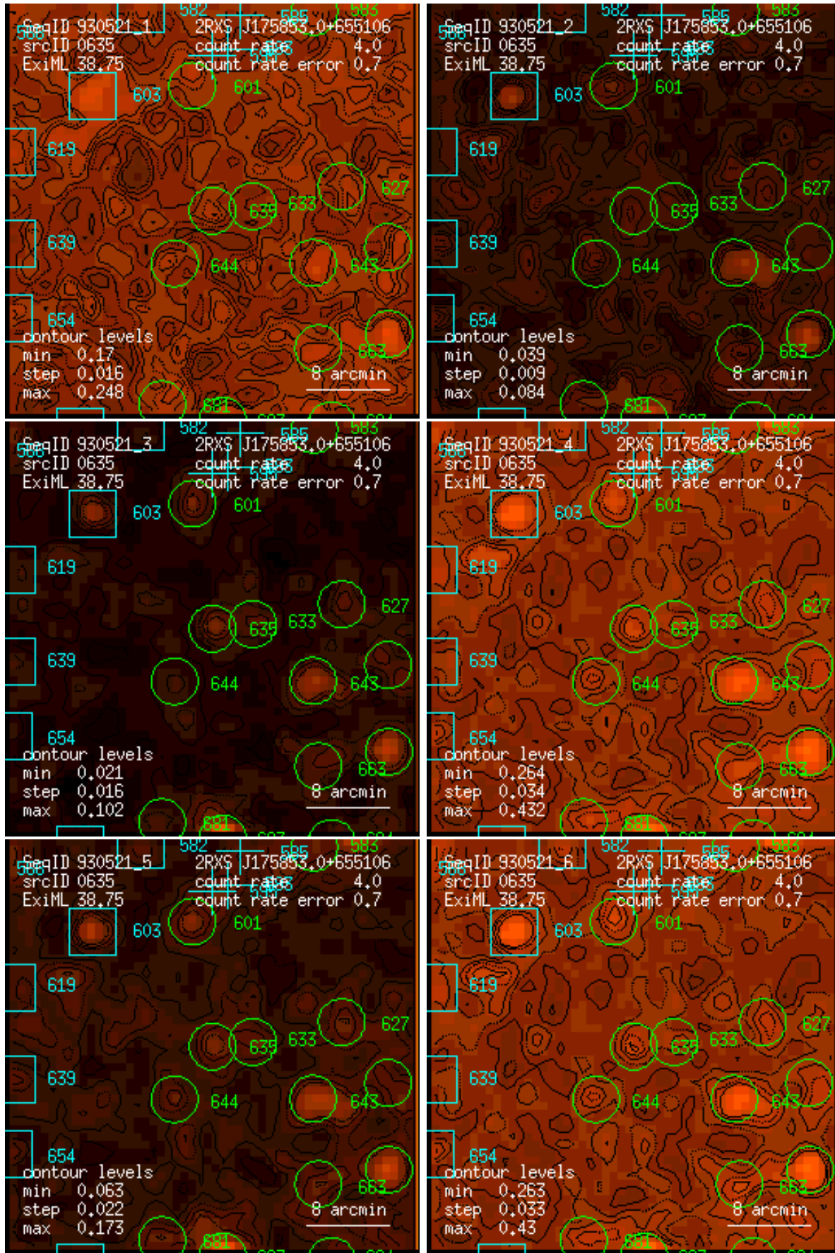
Figure 635: RASS 930521: detection 0635: band rate images, Gaussian filter: (1) PSPC channels 11 – 41, (2) 52 – 90, (3) 91 – 201, (4) 11 – 235, (5) 52 – 201, (6) 11 – 201. Broad band rates in counts/ks. Band rate contour levels in counts/ks/arcmin 2 .
