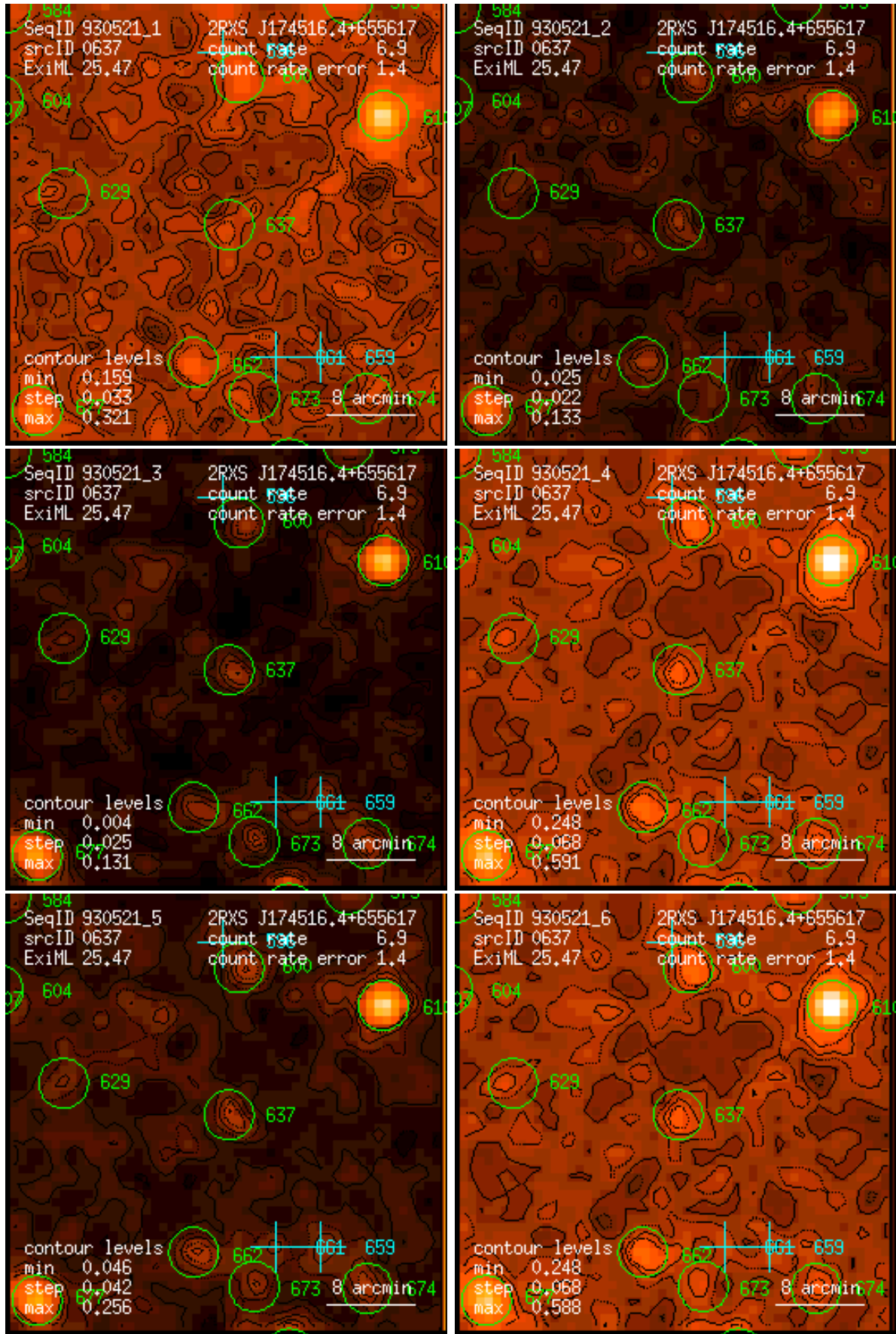
Figure 637: RASS 930521: detection 0637: band rate images, Gaussian filter: (1) PSPC channels 11 – 41, (2) 52 – 90, (3) 91 – 201, (4) 11 – 235, (5) 52 – 201, (6) 11 – 201. Broad band rates in counts/ks. Band rate contour levels in counts/ks/arcmin 2 .
