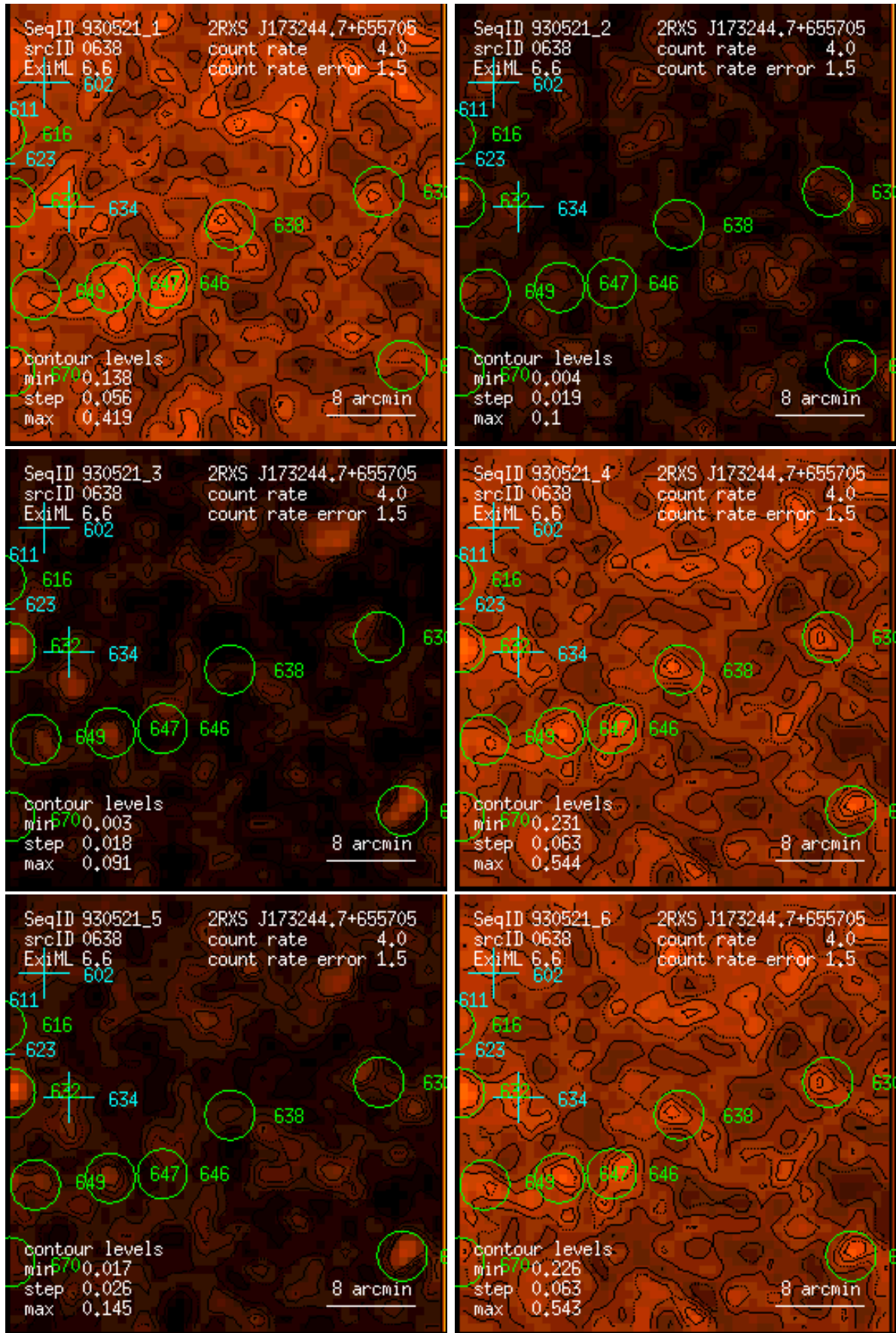
Figure 638: RASS 930521: detection 0638: band rate images, Gaussian filter: (1) PSPC channels 11 – 41, (2) 52 – 90, (3) 91 – 201, (4) 11 – 235, (5) 52 – 201, (6) 11 – 201. Broad band rates in counts/ks. Band rate contour levels in counts/ks/arcmin 2 .
