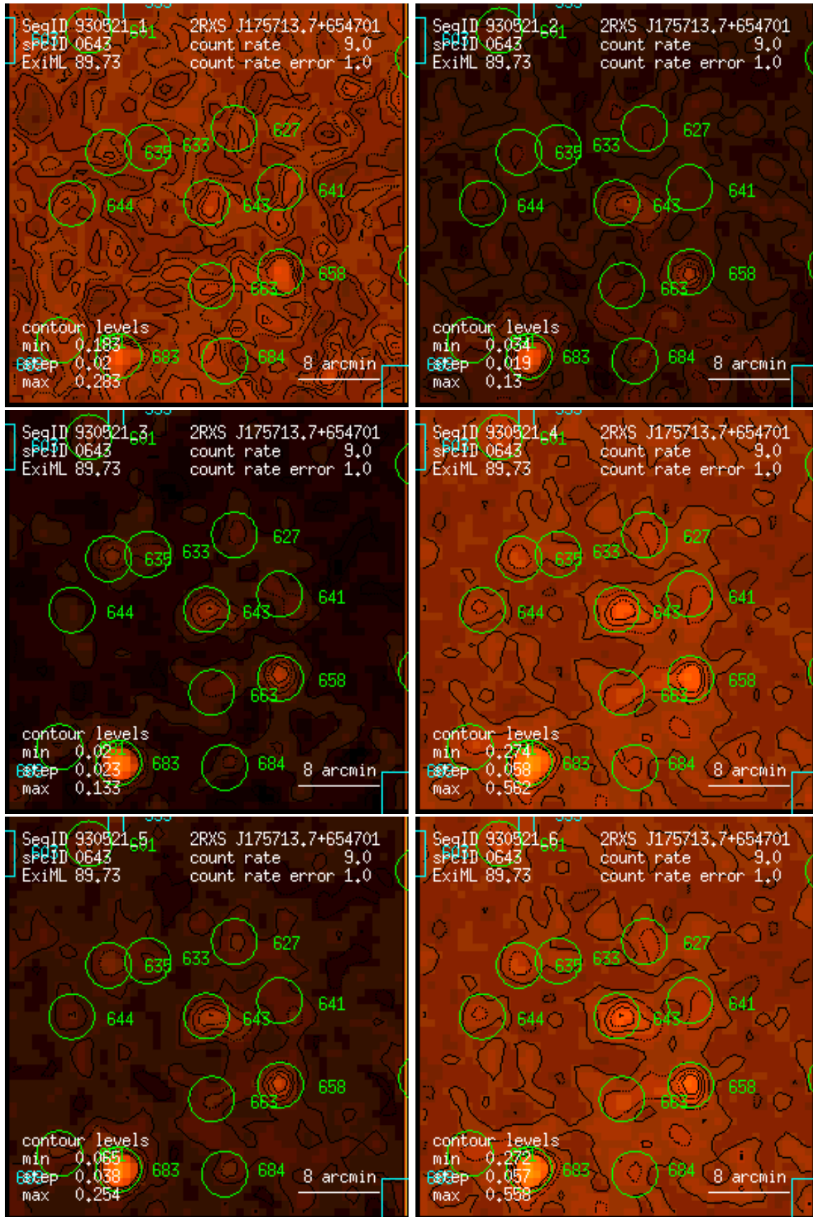
Figure 643: RASS 930521: detection 0643: band rate images, Gaussian filter: (1) PSPC channels 11 – 41, (2) 52 – 90, (3) 91 – 201, (4) 11 – 235, (5) 52 – 201, (6) 11 – 201. Broad band rates in counts/ks. Band rate contour levels in counts/ks/arcmin 2 .
