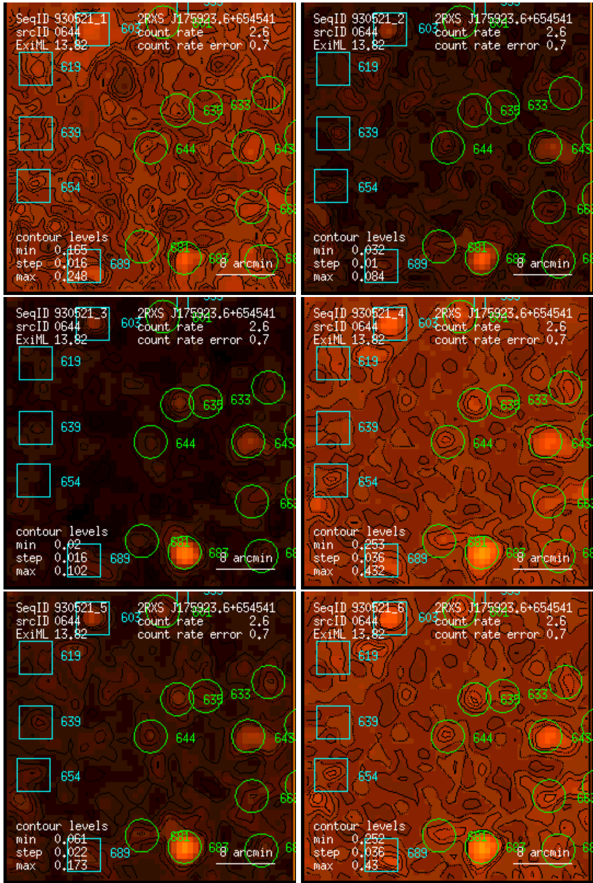
Figure 644: RASS 930521: detection 0644: band rate images, Gaussian filter: (1) PSPC channels 11 – 41, (2) 52 – 90, (3) 91 – 201, (4) 11 – 235, (5) 52 – 201, (6) 11 – 201. Broad band rates in counts/ks. Band rate contour levels in counts/ks/arcmin 2 .
