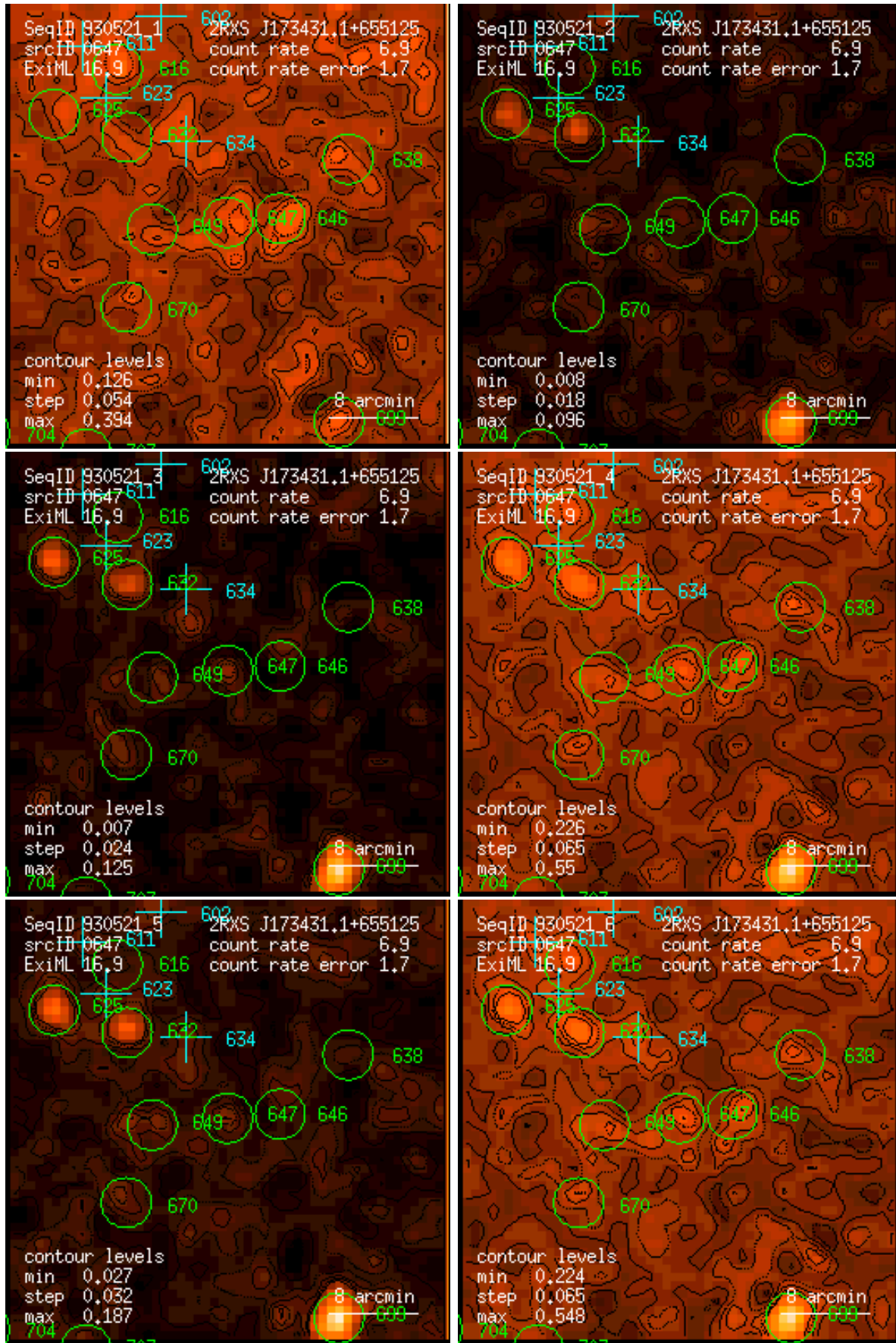
Figure 647: RASS 930521: detection 0647: band rate images, Gaussian filter: (1) PSPC channels 11 – 41, (2) 52 – 90, (3) 91 – 201, (4) 11 – 235, (5) 52 – 201, (6) 11 – 201. Broad band rates in counts/ks. Band rate contour levels in counts/ks/arcmin 2 .
