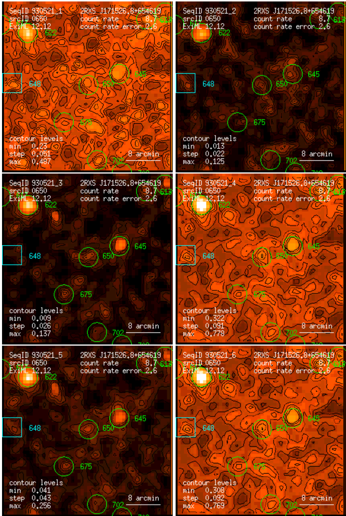
Figure 650: RASS 930521: detection 0650: band rate images, Gaussian filter: (1) PSPC channels 11 – 41, (2) 52 – 90, (3) 91 – 201, (4) 11 – 235, (5) 52 – 201, (6) 11 – 201. Broad band rates in counts/ks. Band rate contour levels in counts/ks/arcmin 2 .
