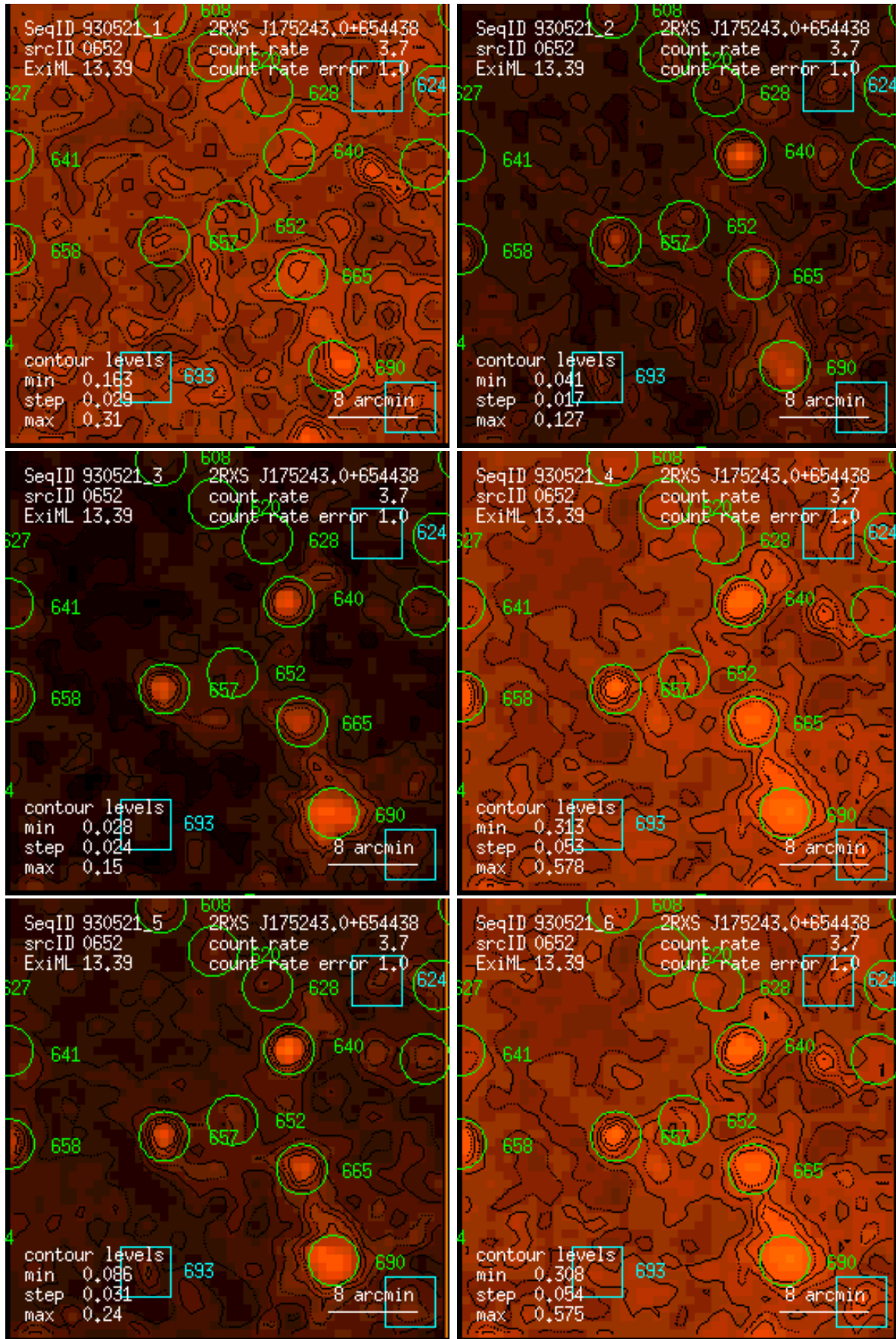
Figure 652: RASS 930521: detection 0652: band rate images, Gaussian filter: (1) PSPC channels 11 – 41, (2) 52 – 90, (3) 91 – 201, (4) 11 – 235, (5) 52 – 201, (6) 11 – 201. Broad band rates in counts/ks. Band rate contour levels in counts/ks/arcmin 2 .
