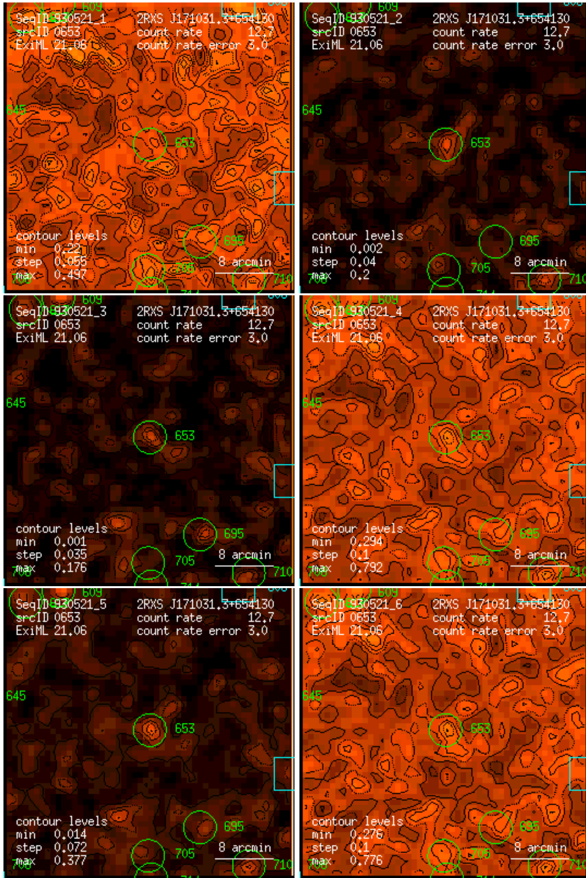
Figure 653: RASS 930521: detection 0653: band rate images, Gaussian filter: (1) PSPC channels 11 – 41, (2) 52 – 90, (3) 91 – 201, (4) 11 – 235, (5) 52 – 201, (6) 11 – 201. Broad band rates in counts/ks. Band rate contour levels in counts/ks/arcmin 2 .
