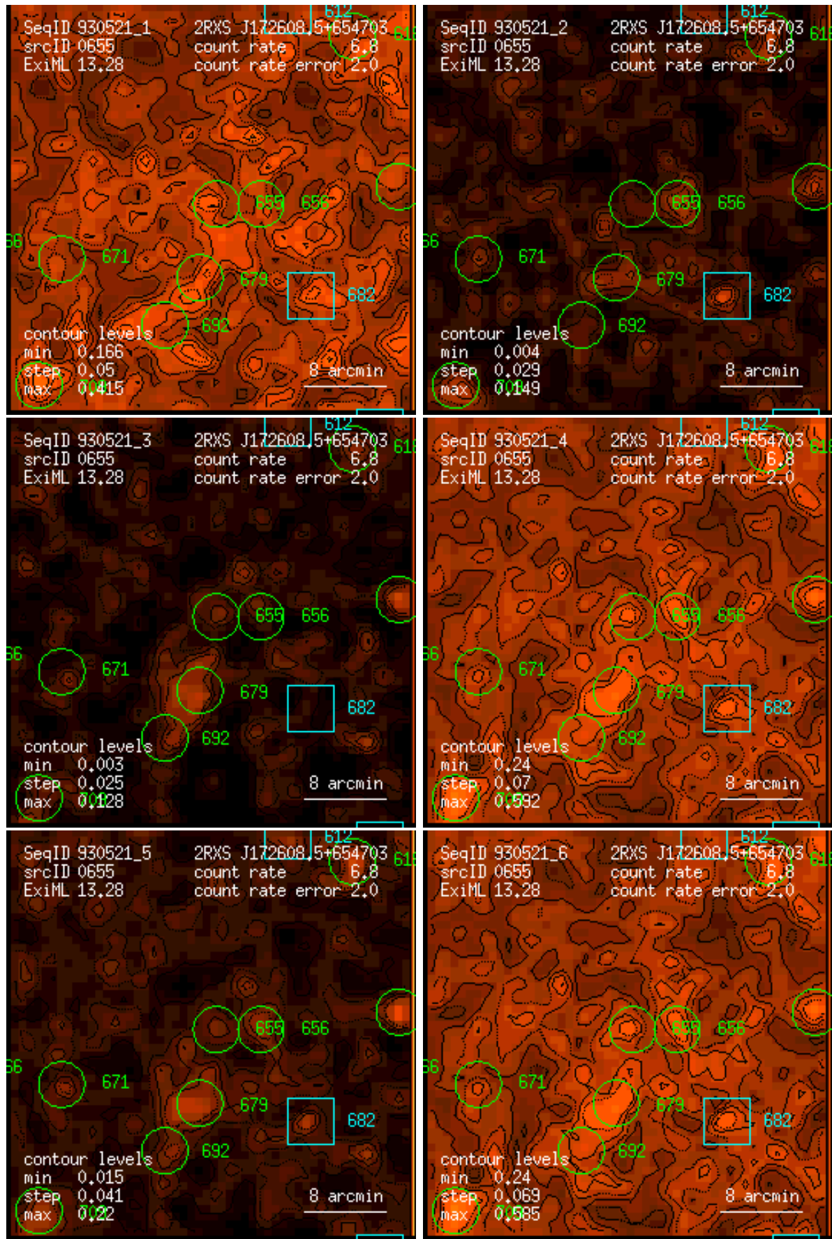
Figure 655: RASS 930521: detection 0655: band rate images, Gaussian filter: (1) PSPC channels 11 – 41, (2) 52 – 90, (3) 91 – 201, (4) 11 – 235, (5) 52 – 201, (6) 11 – 201. Broad band rates in counts/ks. Band rate contour levels in counts/ks/arcmin 2 .
