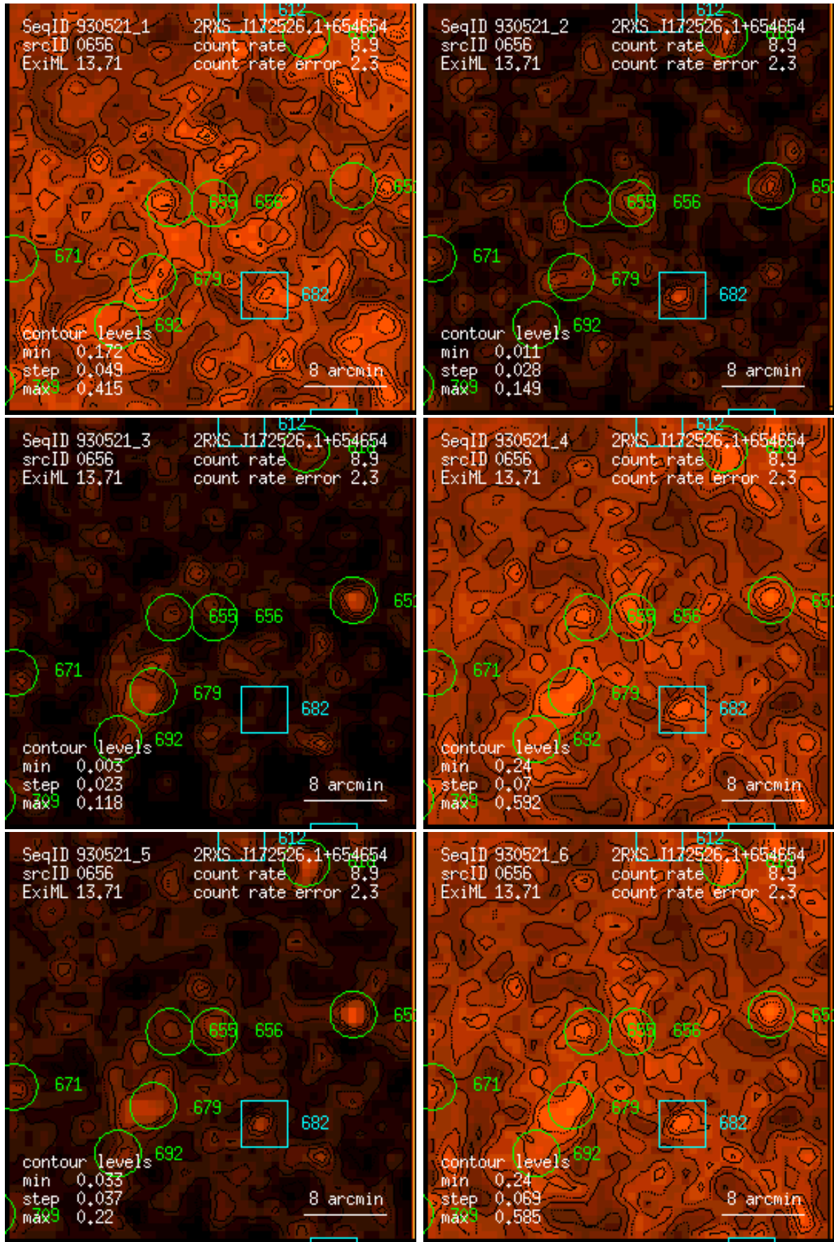
Figure 656: RASS 930521: detection 0656: band rate images, Gaussian filter: (1) PSPC channels 11 – 41, (2) 52 – 90, (3) 91 – 201, (4) 11 – 235, (5) 52 – 201, (6) 11 – 201. Broad band rates in counts/ks. Band rate contour levels in counts/ks/arcmin 2 .
