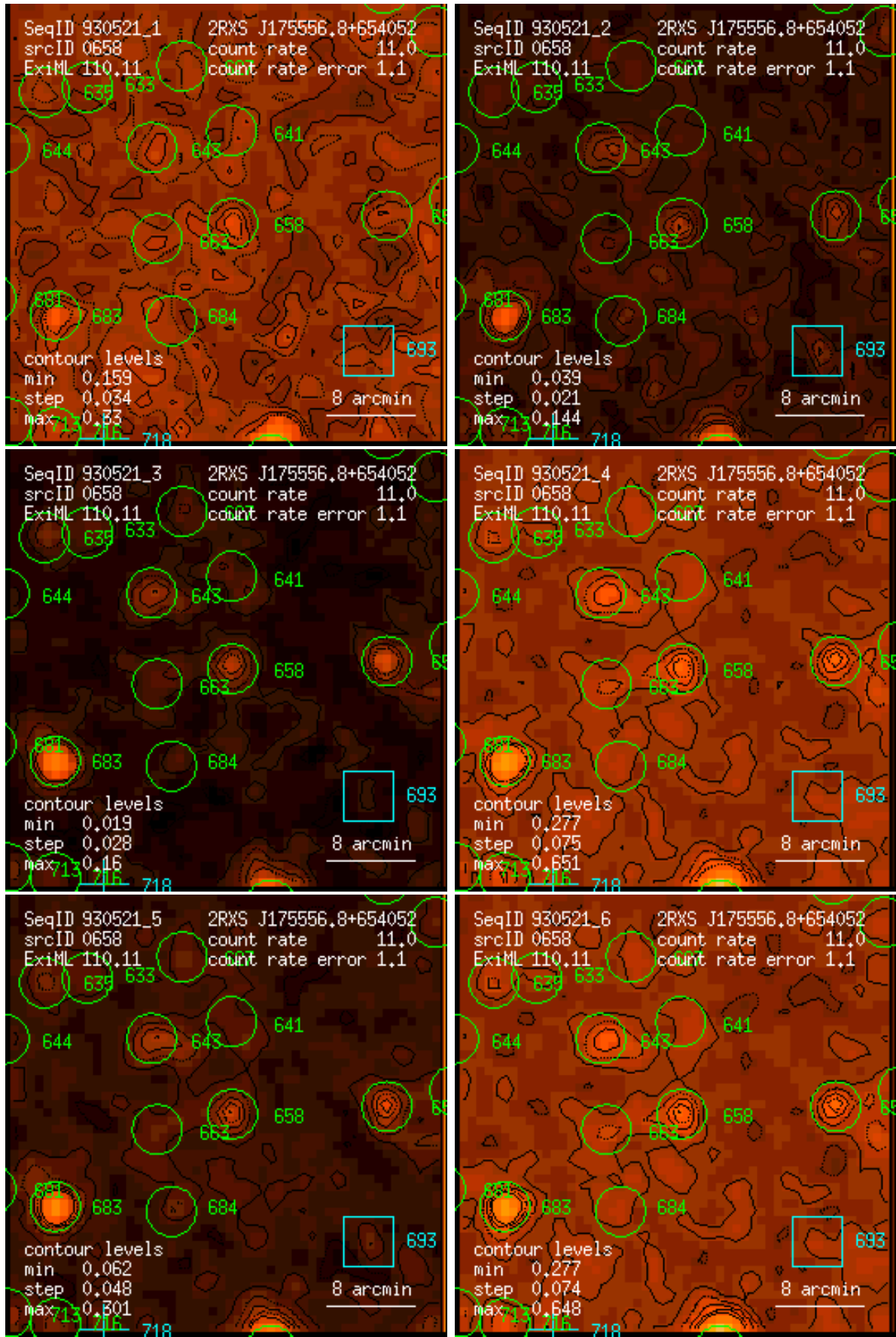
Figure 658: RASS 930521: detection 0658: band rate images, Gaussian filter: (1) PSPC channels 11 – 41, (2) 52 – 90, (3) 91 – 201, (4) 11 – 235, (5) 52 – 201, (6) 11 – 201. Broad band rates in counts/ks. Band rate contour levels in counts/ks/arcmin 2 .
