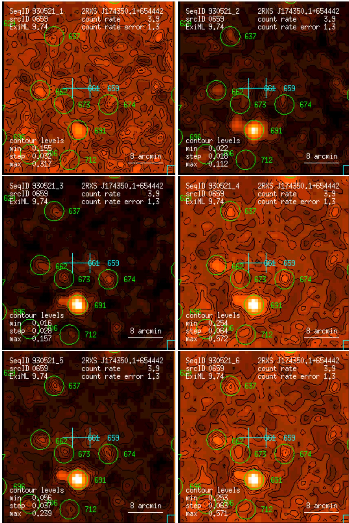
Figure 659: RASS 930521: detection 0659: band rate images, Gaussian filter: (1) PSPC channels 11 – 41, (2) 52 – 90, (3) 91 – 201, (4) 11 – 235, (5) 52 – 201, (6) 11 – 201. Broad band rates in counts/ks. Band rate contour levels in counts/ks/arcmin 2 .
