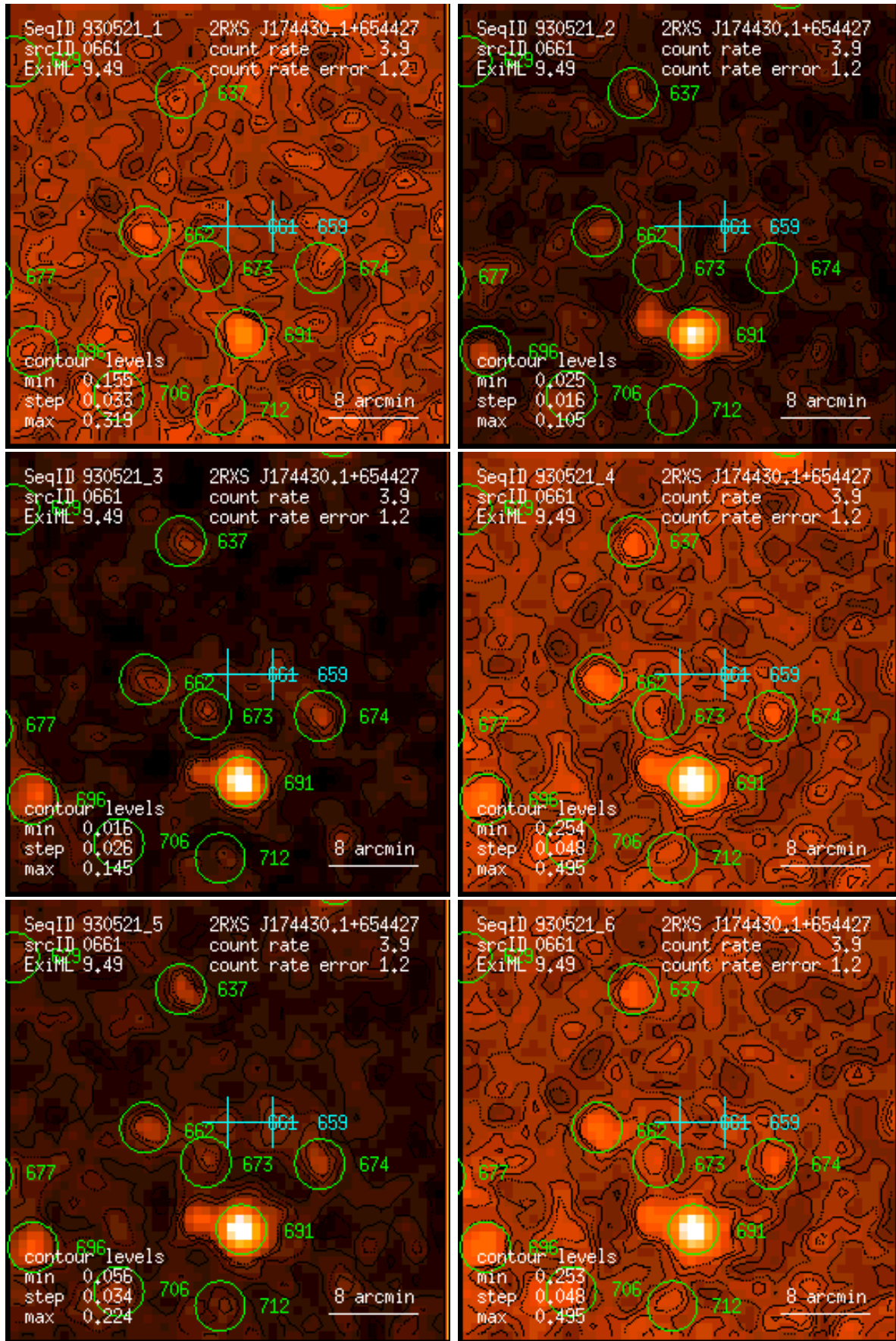
Figure 661: RASS 930521: detection 0661: band rate images, Gaussian filter: (1) PSPC channels 11 – 41, (2) 52 – 90, (3) 91 – 201, (4) 11 – 235, (5) 52 – 201, (6) 11 – 201. Broad band rates in counts/ks. Band rate contour levels in counts/ks/arcmin 2 .
