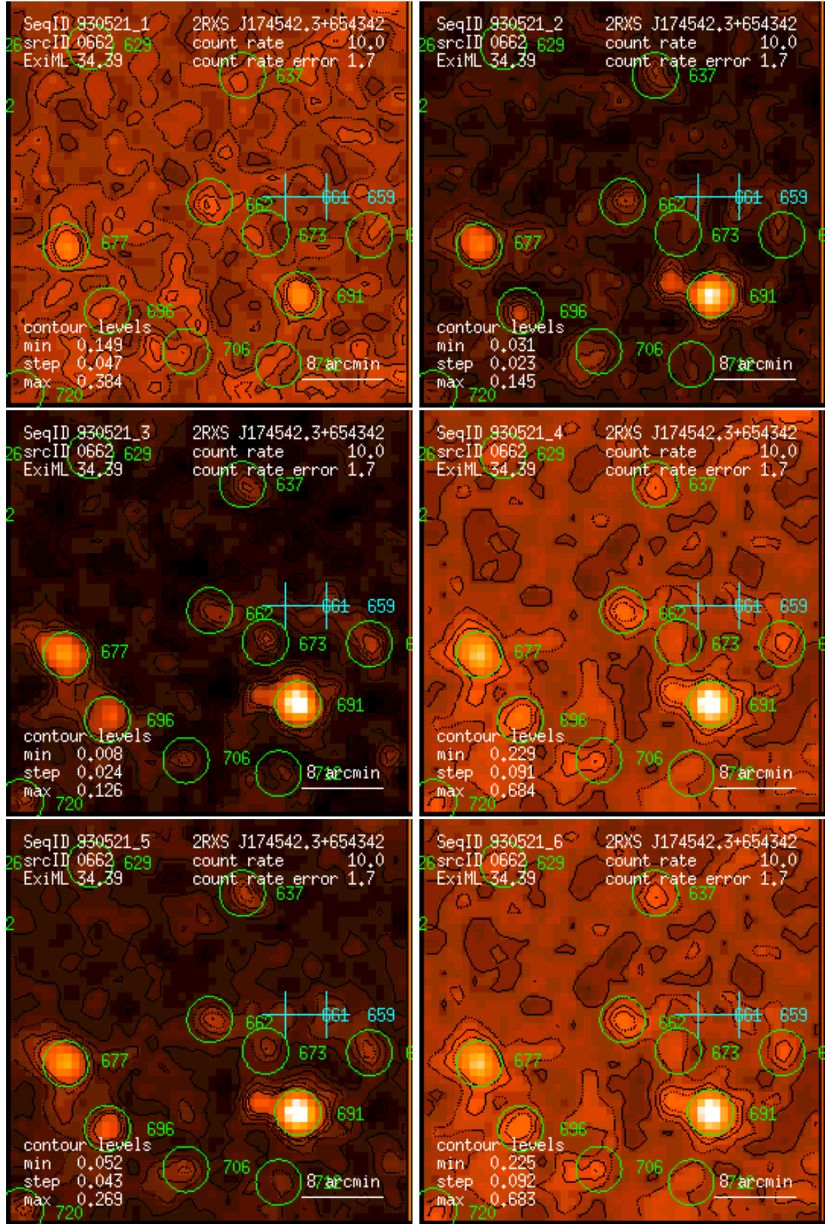
Figure 662: RASS 930521: detection 0662: band rate images, Gaussian filter: (1) PSPC channels 11 – 41, (2) 52 – 90, (3) 91 – 201, (4) 11 – 235, (5) 52 – 201, (6) 11 – 201. Broad band rates in counts/ks. Band rate contour levels in counts/ks/arcmin 2 .
