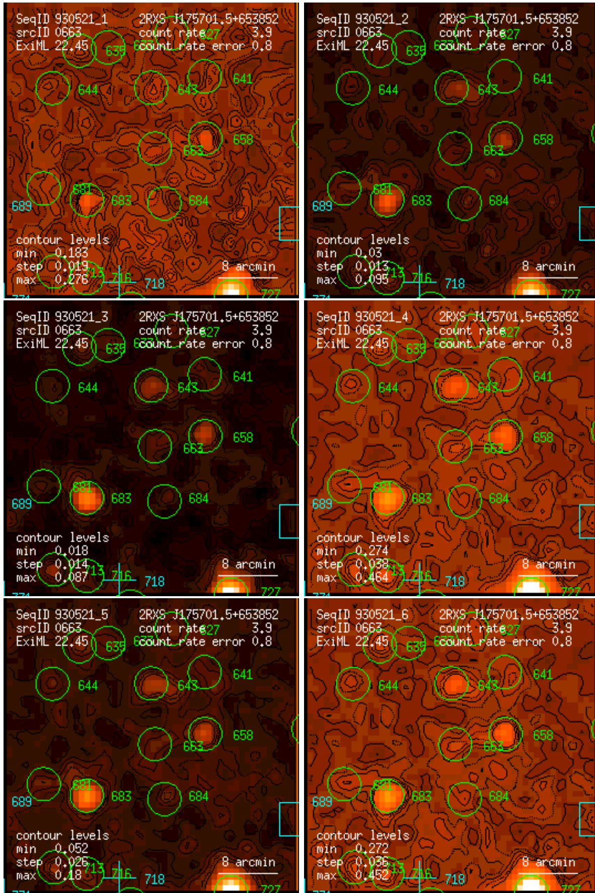
Figure 663: RASS 930521: detection 0663: band rate images, Gaussian filter: (1) PSPC channels 11 – 41, (2) 52 – 90, (3) 91 – 201, (4) 11 – 235, (5) 52 – 201, (6) 11 – 201. Broad band rates in counts/ks. Band rate contour levels in counts/ks/arcmin 2 .
