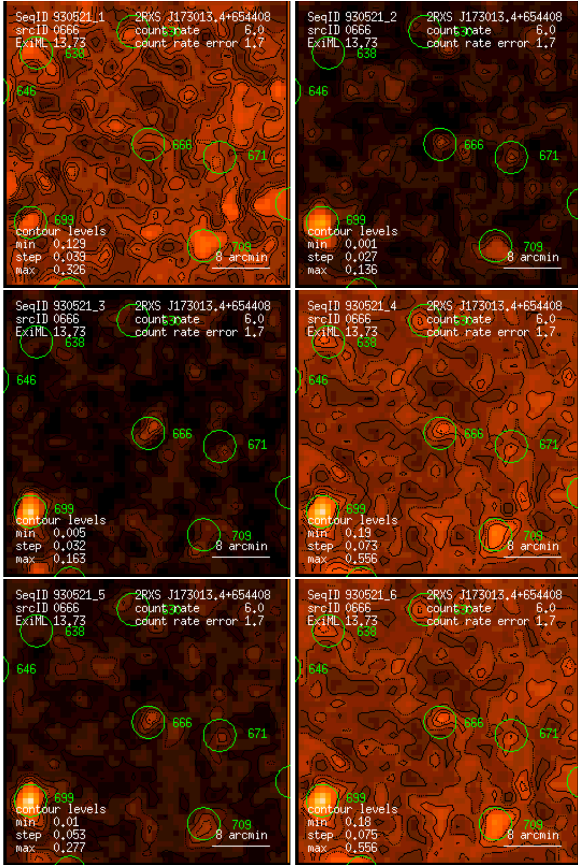
Figure 666: RASS 930521: detection 0666: band rate images, Gaussian filter: (1) PSPC channels 11 – 41, (2) 52 – 90, (3) 91 – 201, (4) 11 – 235, (5) 52 – 201, (6) 11 – 201. Broad band rates in counts/ks. Band rate contour levels in counts/ks/arcmin 2 .
