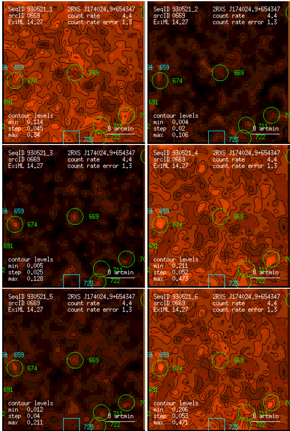
Figure 669: RASS 930521: detection 0669: band rate images, Gaussian filter: (1) PSPC channels 11 – 41, (2) 52 – 90, (3) 91 – 201, (4) 11 – 235, (5) 52 – 201, (6) 11 – 201. Broad band rates in counts/ks. Band rate contour levels in counts/ks/arcmin 2 .
