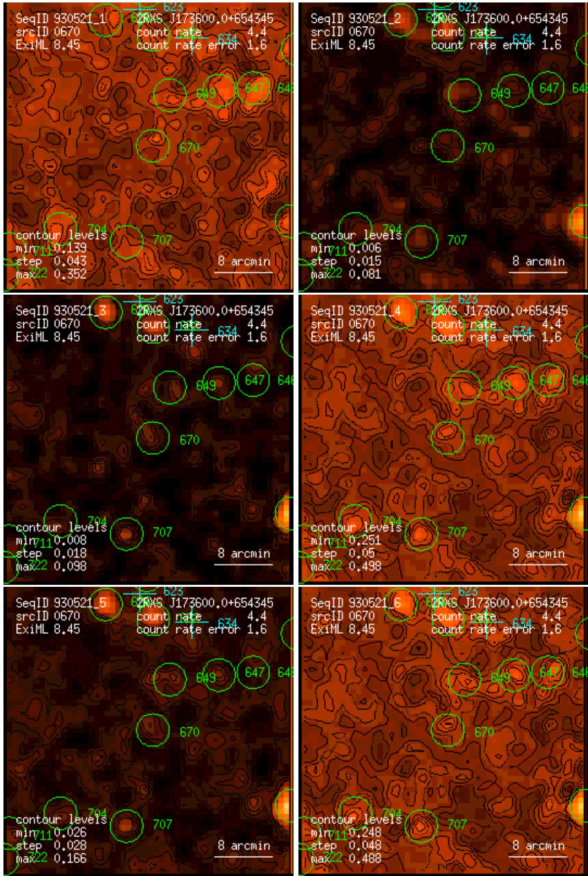
Figure 670: RASS 930521: detection 0670: band rate images, Gaussian filter: (1) PSPC channels 11 – 41, (2) 52 – 90, (3) 91 – 201, (4) 11 – 235, (5) 52 – 201, (6) 11 – 201. Broad band rates in counts/ks. Band rate contour levels in counts/ks/arcmin 2 .
