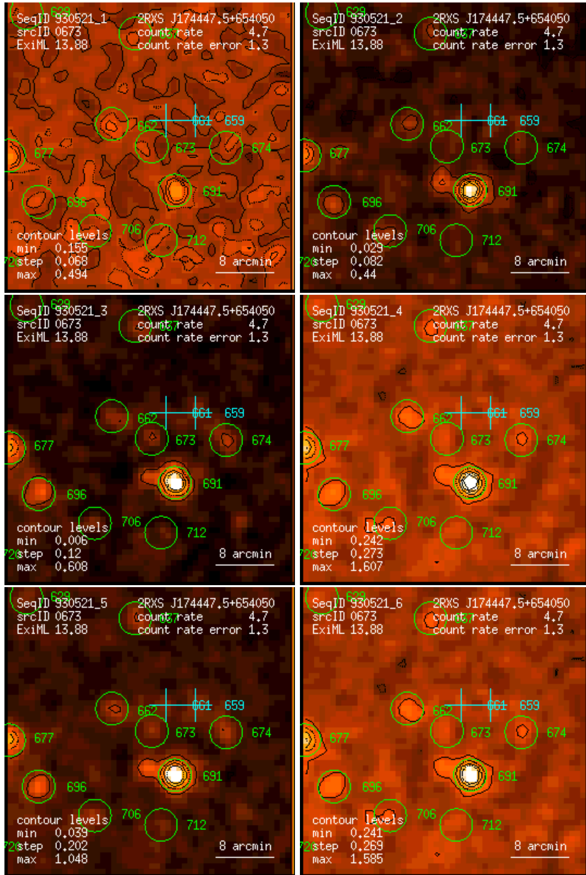
Figure 673: RASS 930521: detection 0673: band rate images, Gaussian filter: (1) PSPC channels 11 – 41, (2) 52 – 90, (3) 91 – 201, (4) 11 – 235, (5) 52 – 201, (6) 11 – 201. Broad band rates in counts/ks. Band rate contour levels in counts/ks/arcmin 2 .
