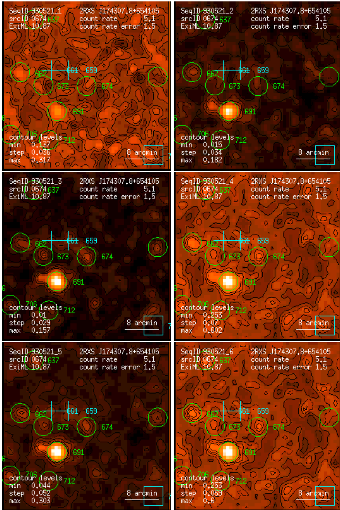
Figure 674: RASS 930521: detection 0674: band rate images, Gaussian filter: (1) PSPC channels 11 – 41, (2) 52 – 90, (3) 91 – 201, (4) 11 – 235, (5) 52 – 201, (6) 11 – 201. Broad band rates in counts/ks. Band rate contour levels in counts/ks/arcmin 2 .
