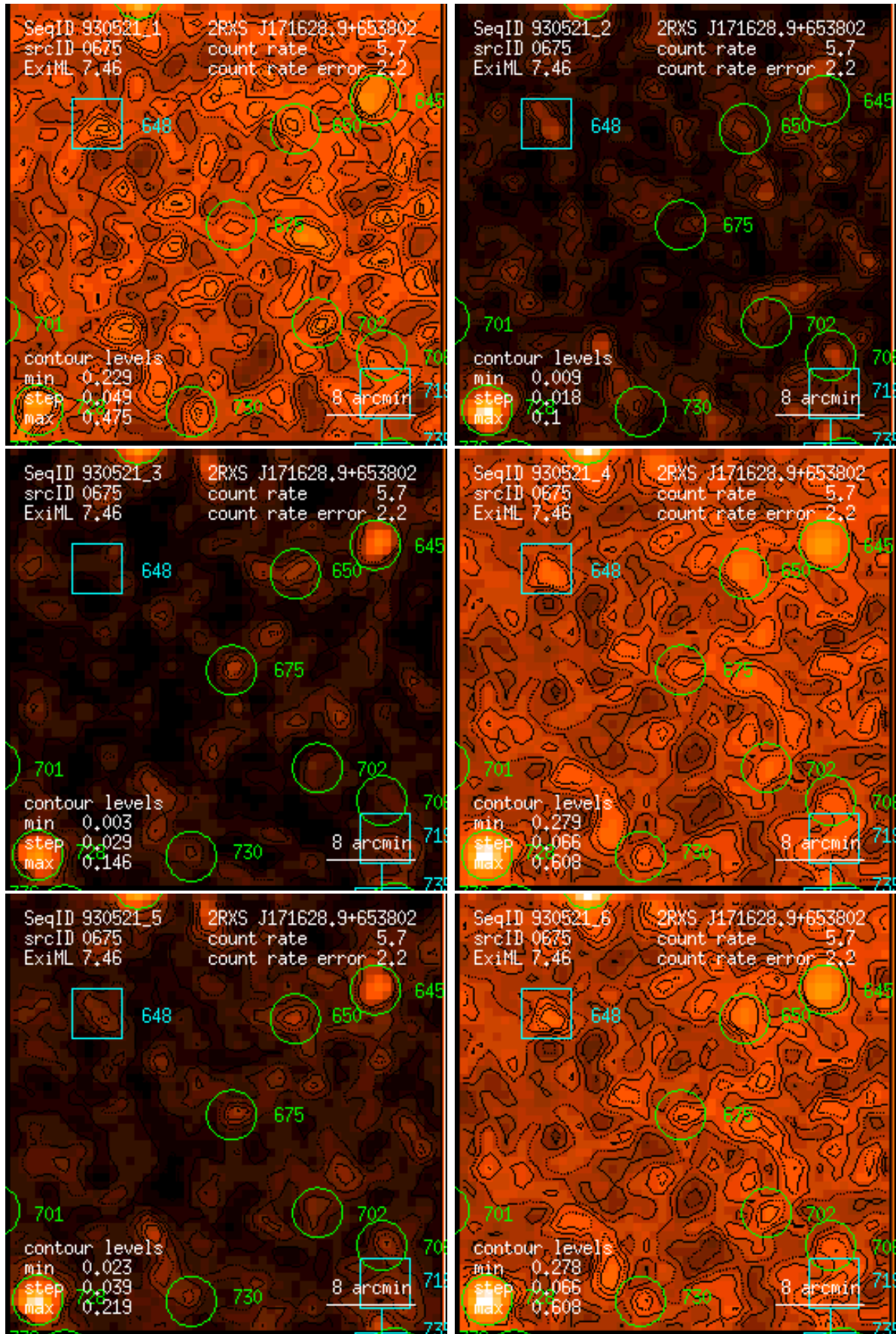
Figure 675: RASS 930521: detection 0675: band rate images, Gaussian filter: (1) PSPC channels 11 – 41, (2) 52 – 90, (3) 91 – 201, (4) 11 – 235, (5) 52 – 201, (6) 11 – 201. Broad band rates in counts/ks. Band rate contour levels in counts/ks/arcmin 2 .
