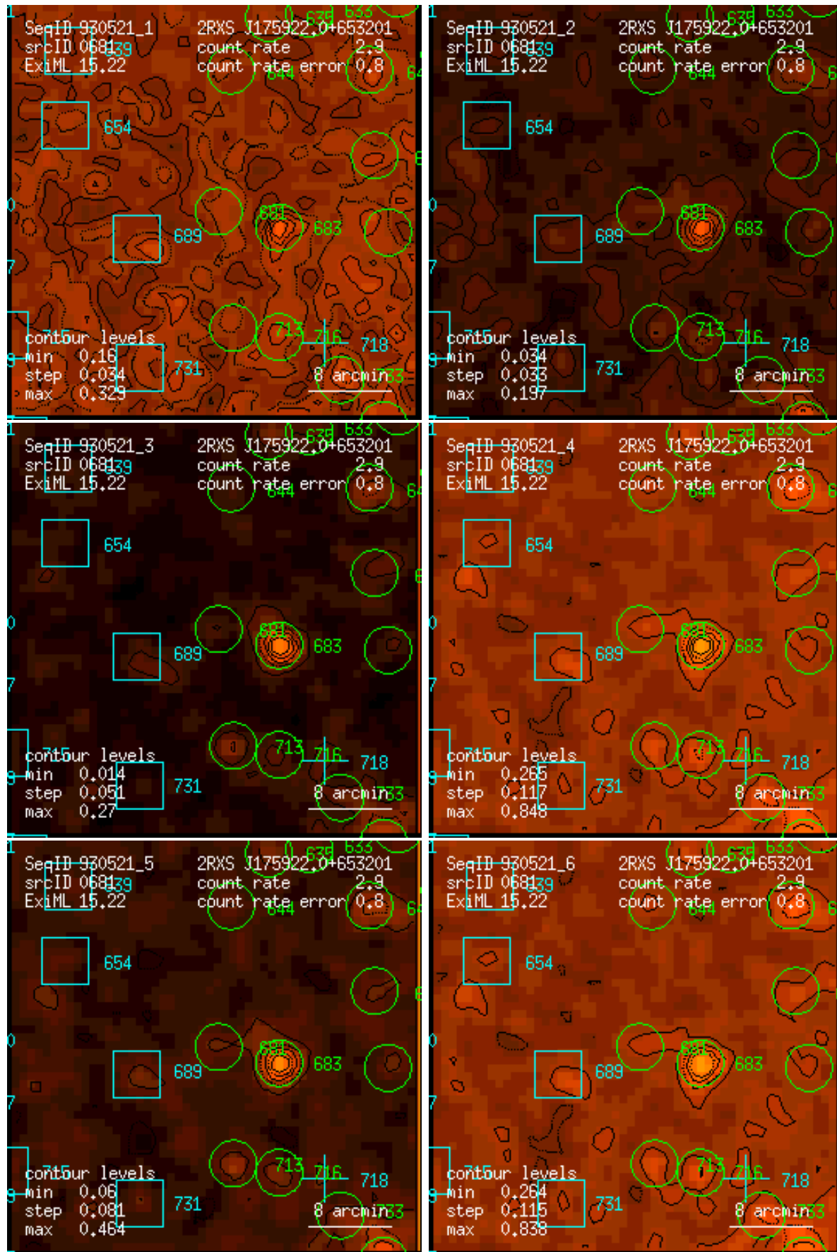
Figure 681: RASS 930521: detection 0681: band rate images, Gaussian filter: (1) PSPC channels 11 – 41, (2) 52 – 90, (3) 91 – 201, (4) 11 – 235, (5) 52 – 201, (6) 11 – 201. Broad band rates in counts/ks. Band rate contour levels in counts/ks/arcmin 2 .
