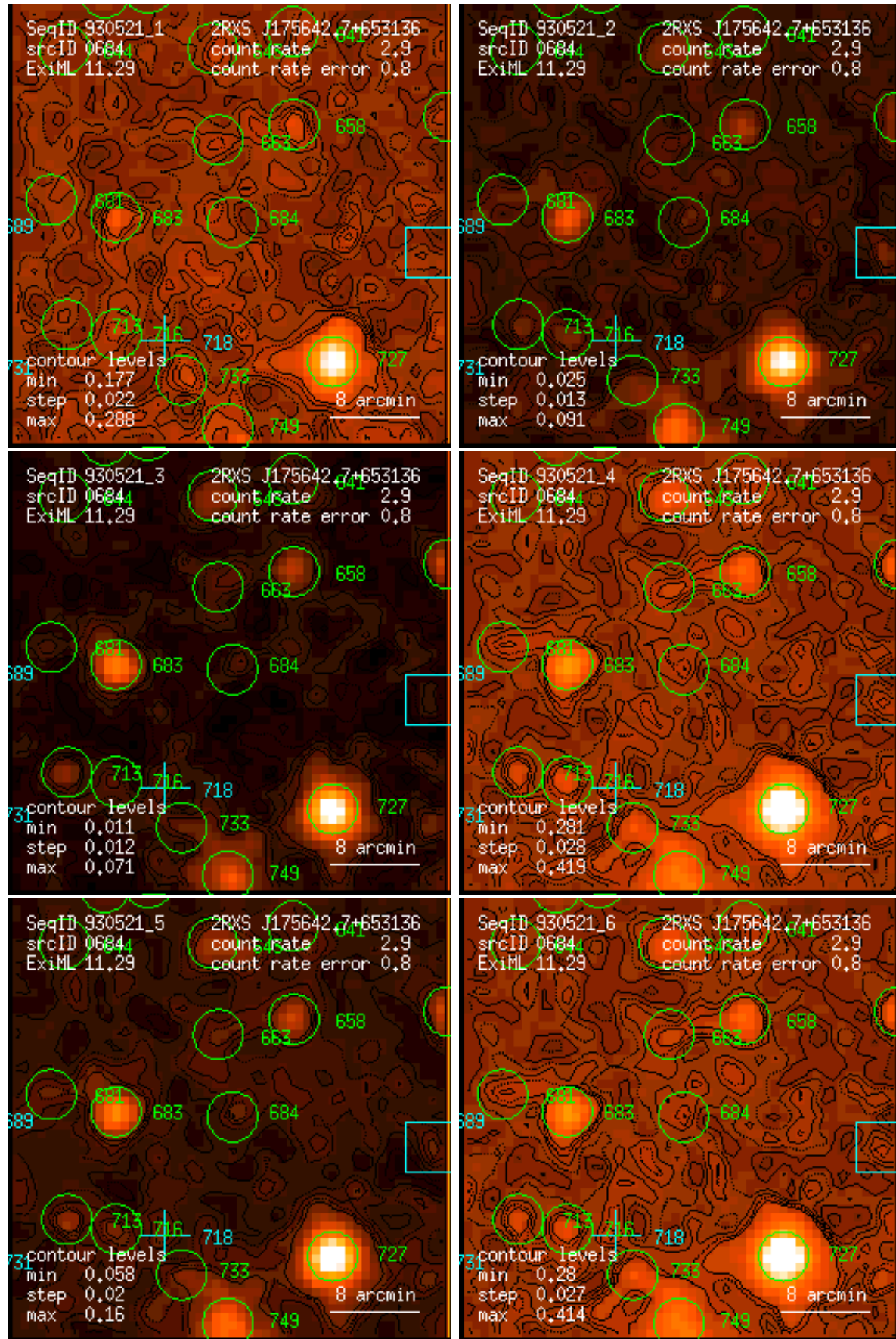
Figure 684: RASS 930521: detection 0684: band rate images, Gaussian filter: (1) PSPC channels 11 – 41, (2) 52 – 90, (3) 91 – 201, (4) 11 – 235, (5) 52 – 201, (6) 11 – 201. Broad band rates in counts/ks. Band rate contour levels in counts/ks/arcmin 2 .
