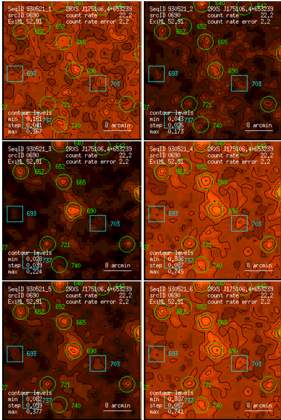
Figure 690: RASS 930521: detection 0690: band rate images, Gaussian filter: (1) PSPC channels 11 – 41, (2) 52 – 90, (3) 91 – 201, (4) 11 – 235, (5) 52 – 201, (6) 11 – 201. Broad band rates in counts/ks. Band rate contour levels in counts/ks/arcmin 2 .
