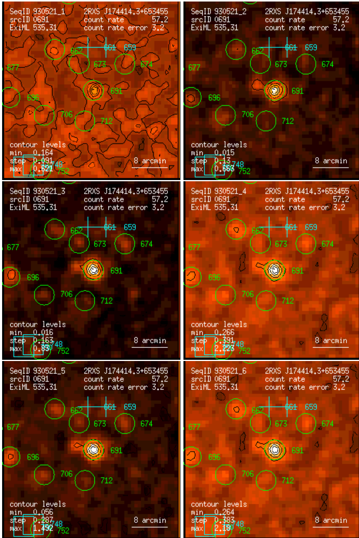
Figure 691: RASS 930521: detection 0691: band rate images, Gaussian filter: (1) PSPC channels 11 – 41, (2) 52 – 90, (3) 91 – 201, (4) 11 – 235, (5) 52 – 201, (6) 11 – 201. Broad band rates in counts/ks. Band rate contour levels in counts/ks/arcmin 2 .
