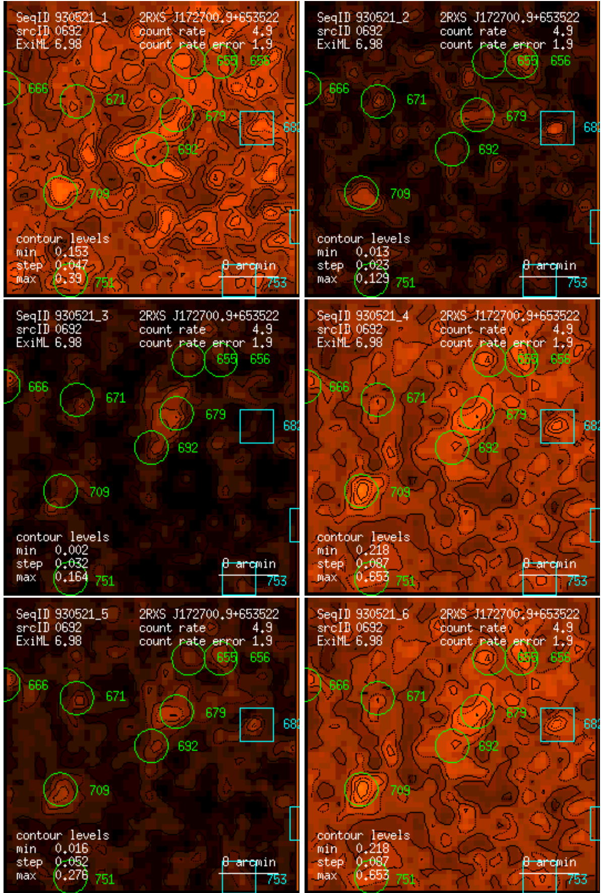
Figure 692: RASS 930521: detection 0692: band rate images, Gaussian filter: (1) PSPC channels 11 – 41, (2) 52 – 90, (3) 91 – 201, (4) 11 – 235, (5) 52 – 201, (6) 11 – 201. Broad band rates in counts/ks. Band rate contour levels in counts/ks/arcmin 2 .
