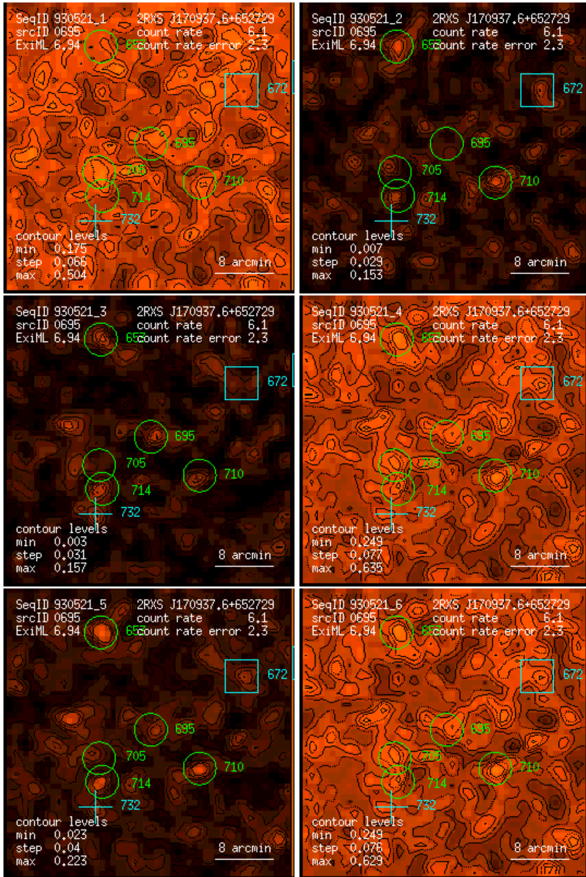
Figure 695: RASS 930521: detection 0695: band rate images, Gaussian filter: (1) PSPC channels 11 – 41, (2) 52 – 90, (3) 91 – 201, (4) 11 – 235, (5) 52 – 201, (6) 11 – 201. Broad band rates in counts/ks. Band rate contour levels in counts/ks/arcmin 2 .
