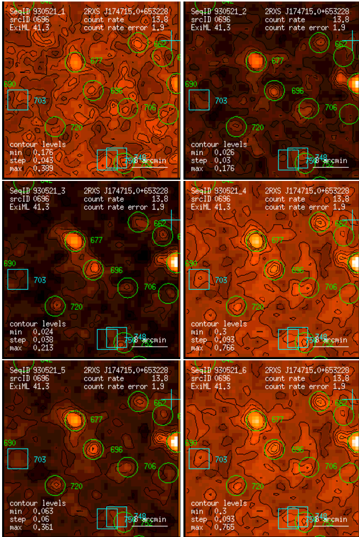
Figure 696: RASS 930521: detection 0696: band rate images, Gaussian filter: (1) PSPC channels 11 – 41, (2) 52 – 90, (3) 91 – 201, (4) 11 – 235, (5) 52 – 201, (6) 11 – 201. Broad band rates in counts/ks. Band rate contour levels in counts/ks/arcmin 2 .
