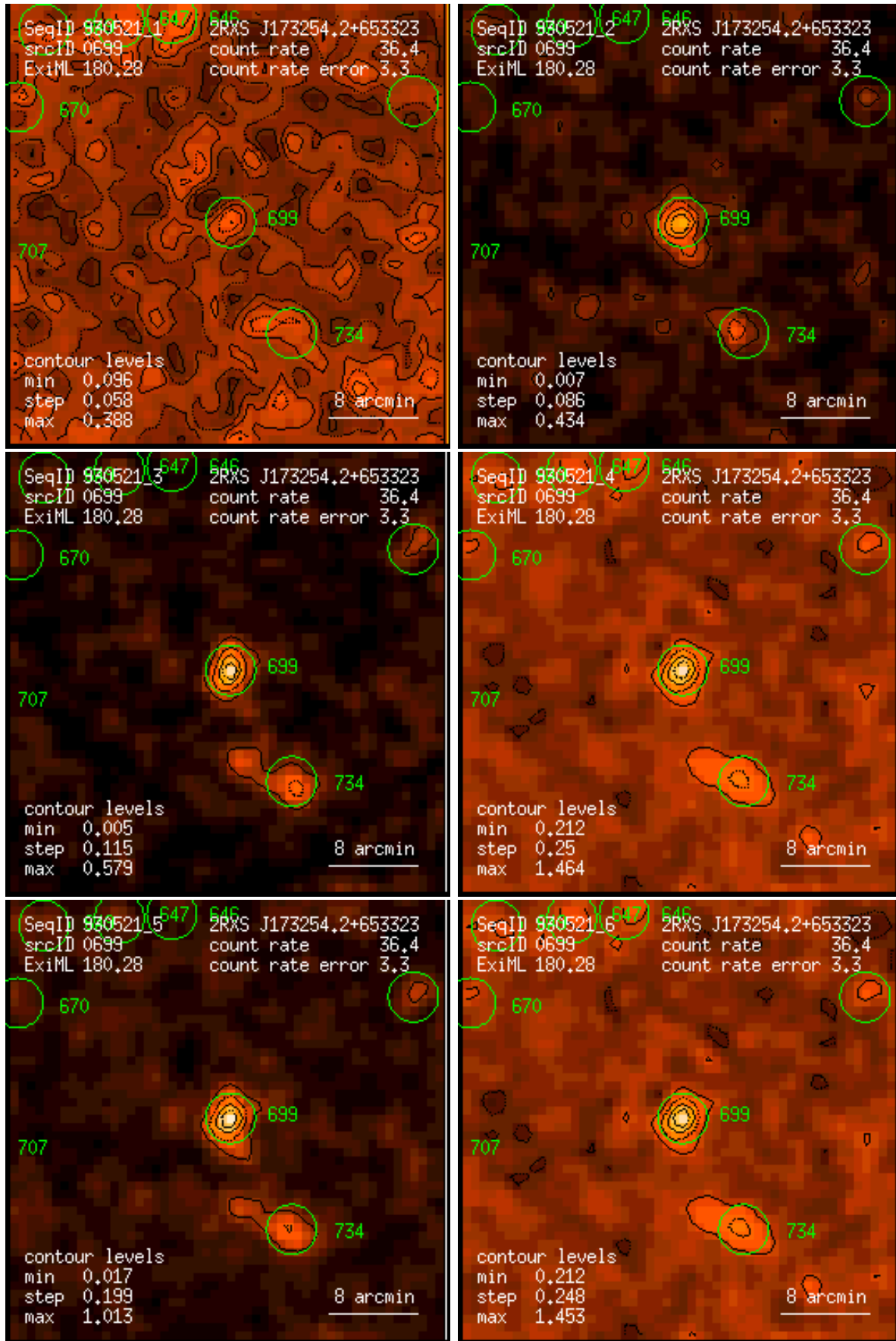
Figure 699: RASS 930521: detection 0699: band rate images, Gaussian filter: (1) PSPC channels 11 – 41, (2) 52 – 90, (3) 91 – 201, (4) 11 – 235, (5) 52 – 201, (6) 11 – 201. Broad band rates in counts/ks. Band rate contour levels in counts/ks/arcmin 2 .
