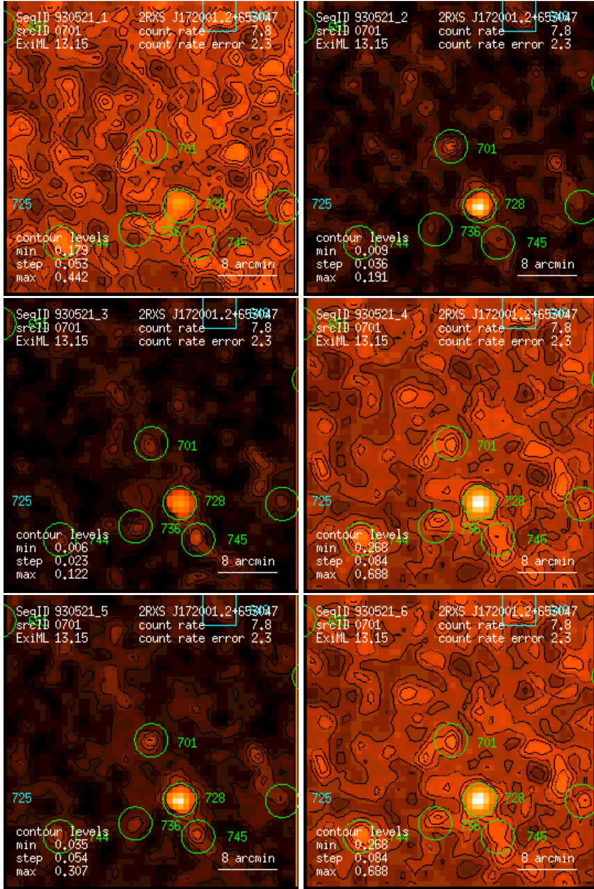
Figure 701: RASS 930521: detection 0701: band rate images, Gaussian filter: (1) PSPC channels 11 – 41, (2) 52 – 90, (3) 91 – 201, (4) 11 – 235, (5) 52 – 201, (6) 11 – 201. Broad band rates in counts/ks. Band rate contour levels in counts/ks/arcmin 2 .
