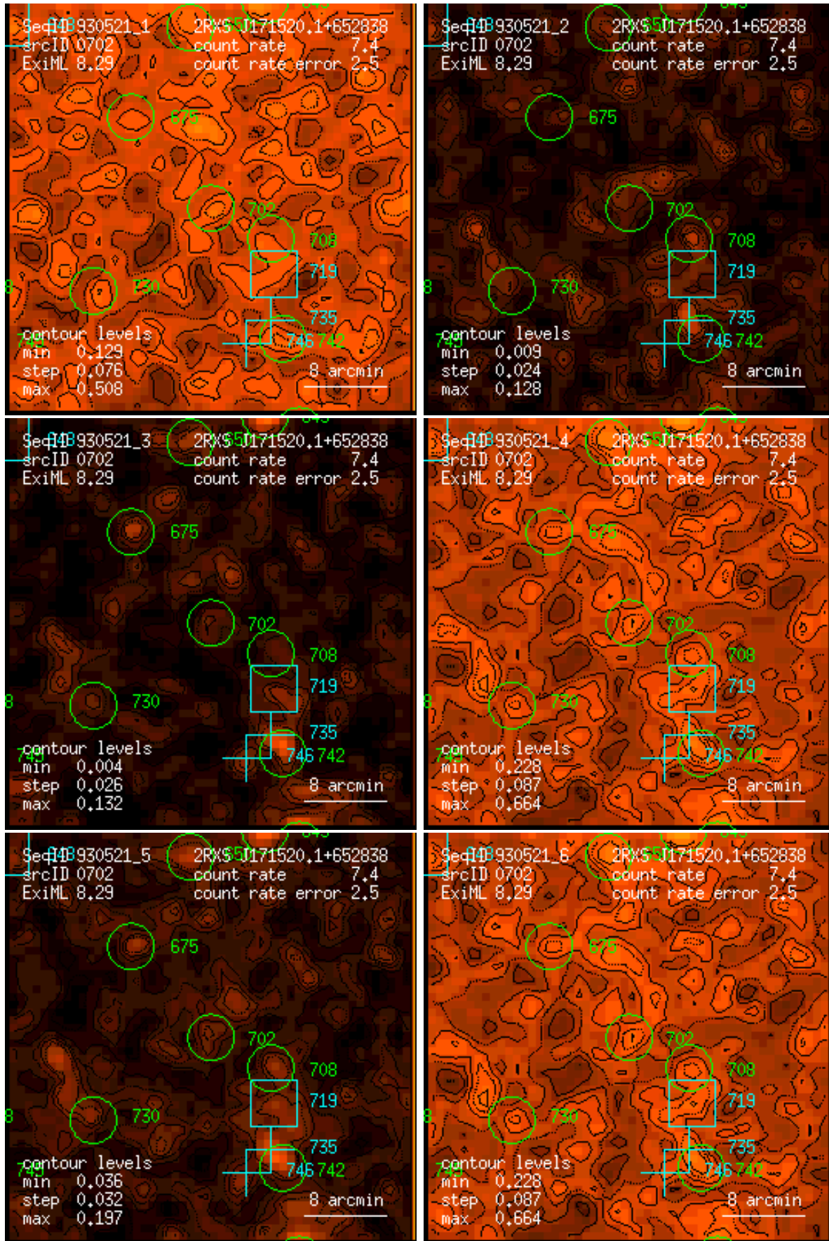
Figure 702: RASS 930521: detection 0702: band rate images, Gaussian filter: (1) PSPC channels 11 – 41, (2) 52 – 90, (3) 91 – 201, (4) 11 – 235, (5) 52 – 201, (6) 11 – 201. Broad band rates in counts/ks. Band rate contour levels in counts/ks/arcmin 2 .
