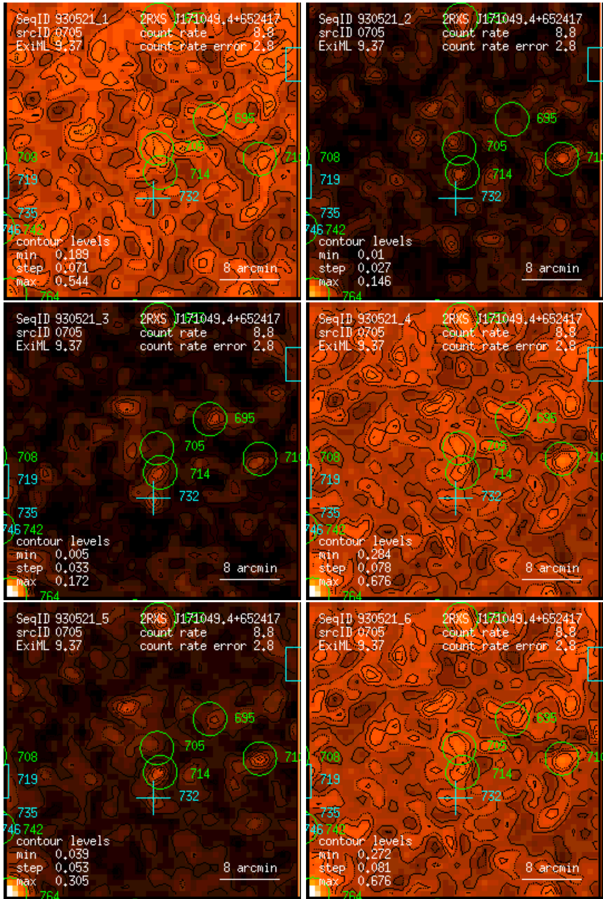
Figure 705: RASS 930521: detection 0705: band rate images, Gaussian filter: (1) PSPC channels 11 – 41, (2) 52 – 90, (3) 91 – 201, (4) 11 – 235, (5) 52 – 201, (6) 11 – 201. Broad band rates in counts/ks. Band rate contour levels in counts/ks/arcmin 2 .
