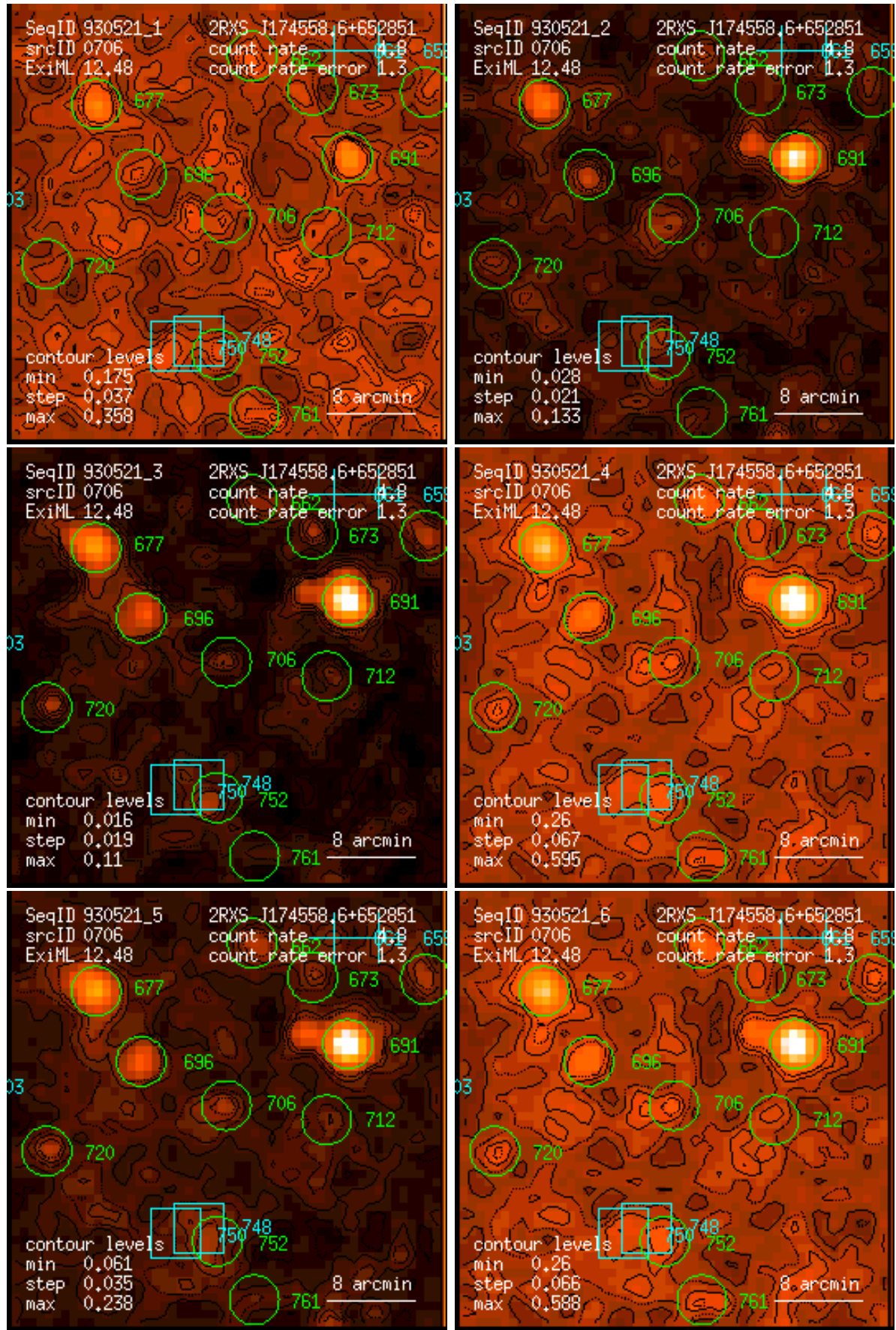
Figure 706: RASS 930521: detection 0706: band rate images, Gaussian filter: (1) PSPC channels 11 – 41, (2) 52 – 90, (3) 91 – 201, (4) 11 – 235, (5) 52 – 201, (6) 11 – 201. Broad band rates in counts/ks. Band rate contour levels in counts/ks/arcmin 2 .
