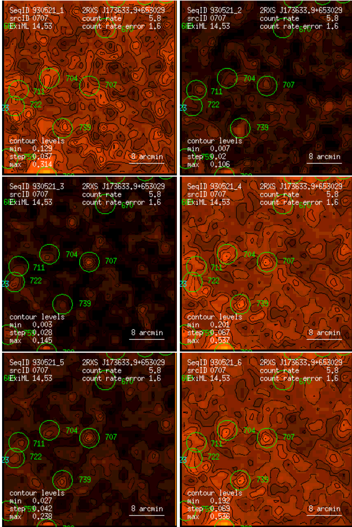
Figure 707: RASS 930521: detection 0707: band rate images, Gaussian filter: (1) PSPC channels 11 – 41, (2) 52 – 90, (3) 91 – 201, (4) 11 – 235, (5) 52 – 201, (6) 11 – 201. Broad band rates in counts/ks. Band rate contour levels in counts/ks/arcmin 2 .
