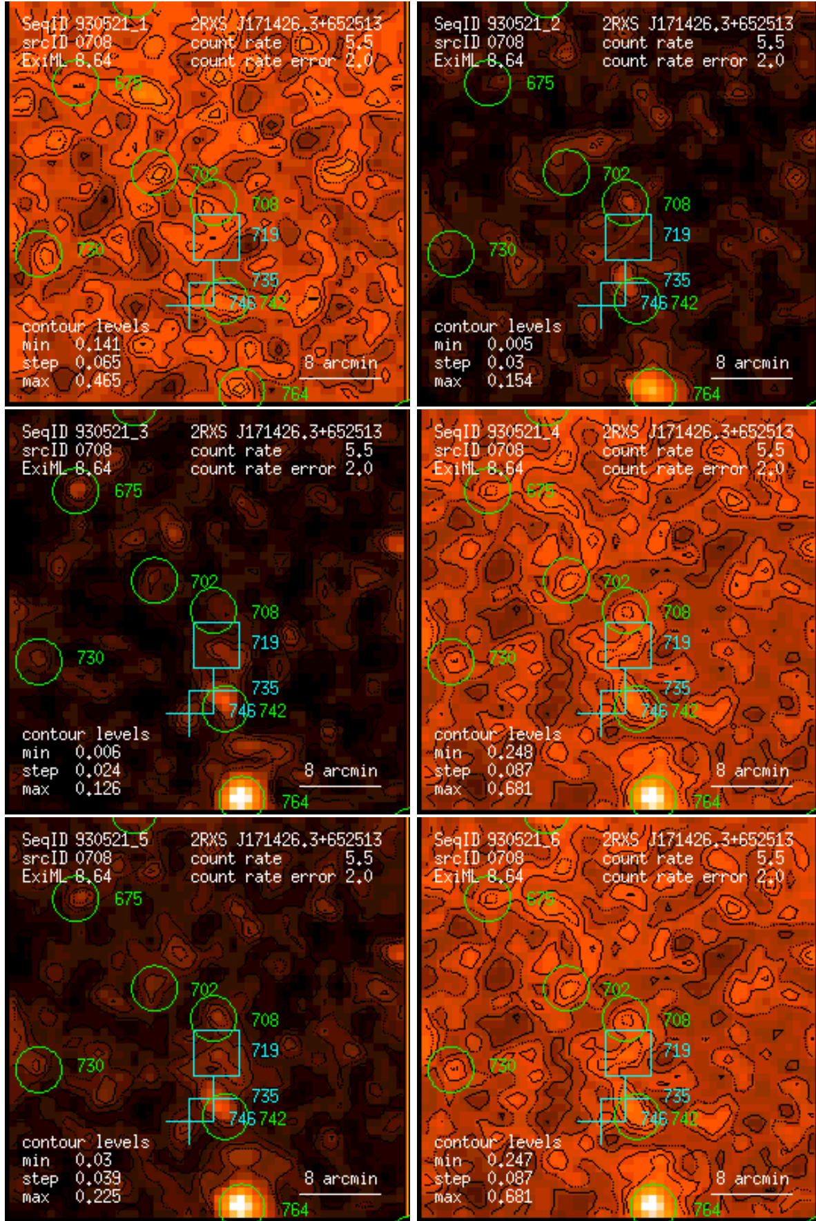
Figure 708: RASS 930521: detection 0708: band rate images, Gaussian filter: (1) PSPC channels 11 – 41, (2) 52 – 90, (3) 91 – 201, (4) 11 – 235, (5) 52 – 201, (6) 11 – 201. Broad band rates in counts/ks. Band rate contour levels in counts/ks/arcmin 2 .
