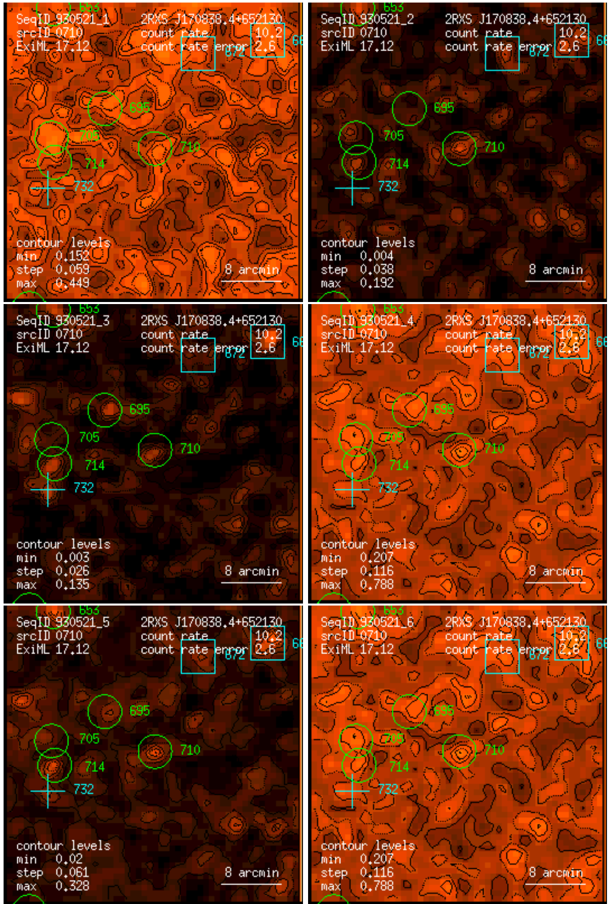
Figure 710: RASS 930521: detection 0710: band rate images, Gaussian filter: (1) PSPC channels 11 – 41, (2) 52 – 90, (3) 91 – 201, (4) 11 – 235, (5) 52 – 201, (6) 11 – 201. Broad band rates in counts/ks. Band rate contour levels in counts/ks/arcmin 2 .
